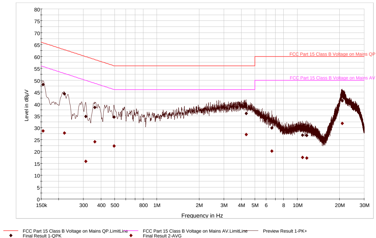
Plot 6-23. Line Conducted Data with Bluetooth (N)
