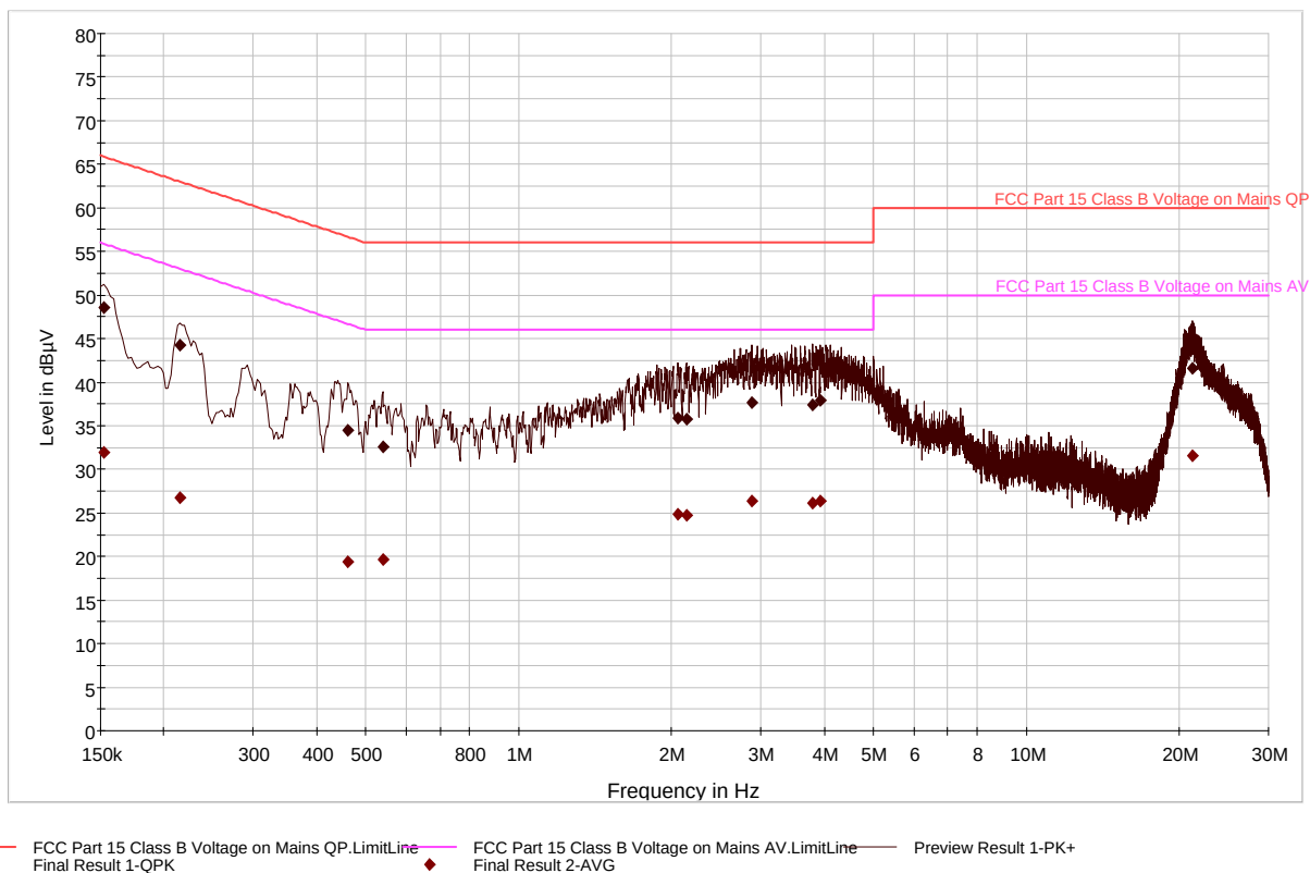
Plot 6-22. Line Conducted Data with Bluetooth (L1)
