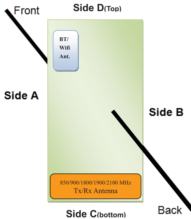
Figure 5.7 Identification of Sides for SAR Testing
