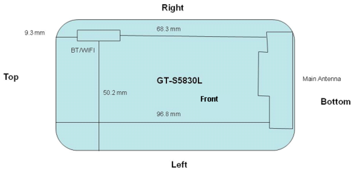
Figure 13-1 Identification of Sides for SAR Testing
