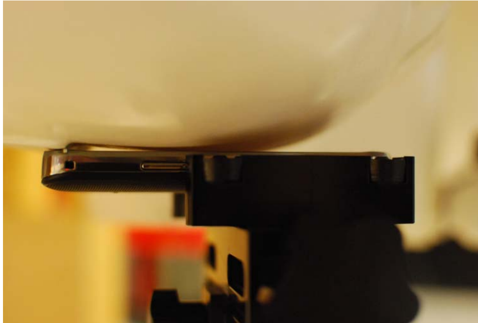
Figure 21-1 SAR Test Setup Photo 1: Right Touch
