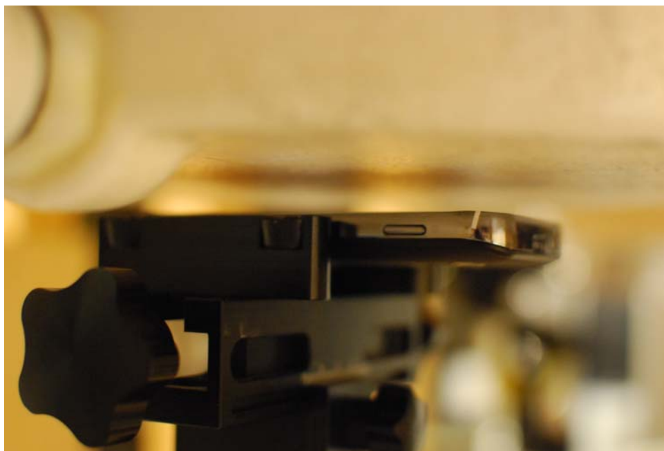
Figure 21-6 SAR Test Setup Photo 6: Front at 1.0 cm
