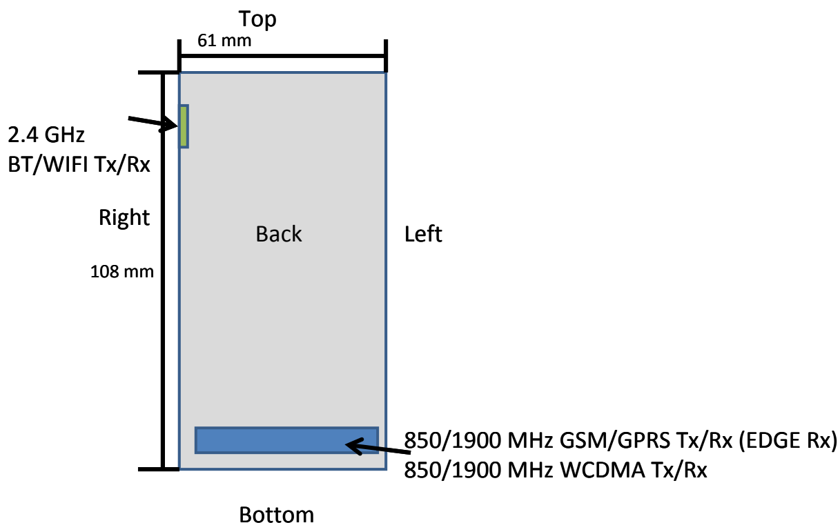
Figure 13-1 Identification of Sides for SAR Testing
