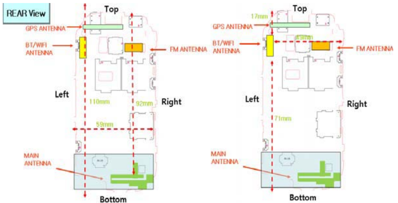
Figure 5.7 Identification of Sides for SAR Testing
