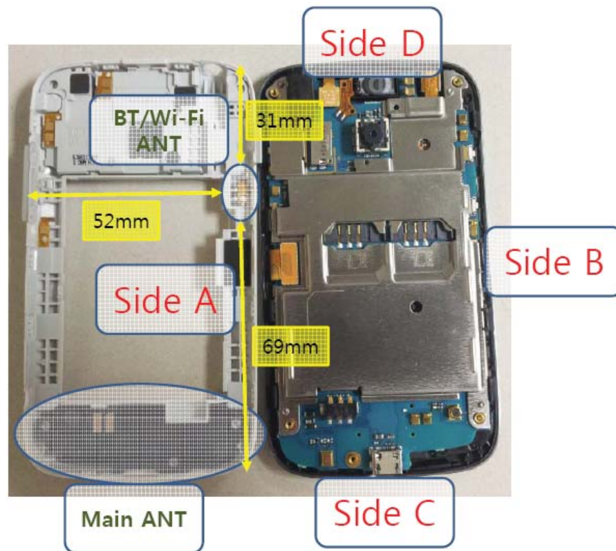
Figure 5.7 Identification of Sides for SAR Testing
