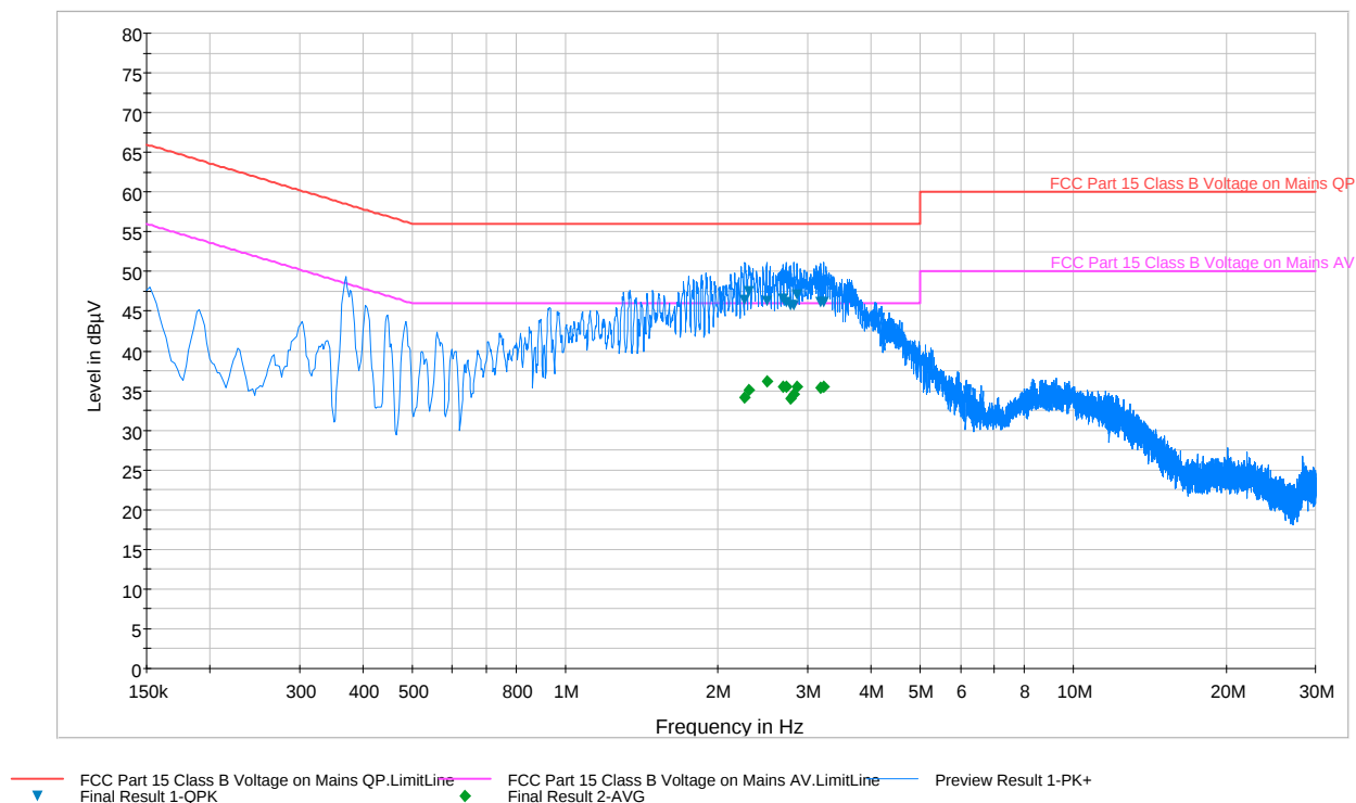
Plot 6-32. Line Conducted Plot with 802.11b
