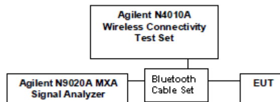
Figure 6-2. Test Instrument & Measurement Setup
