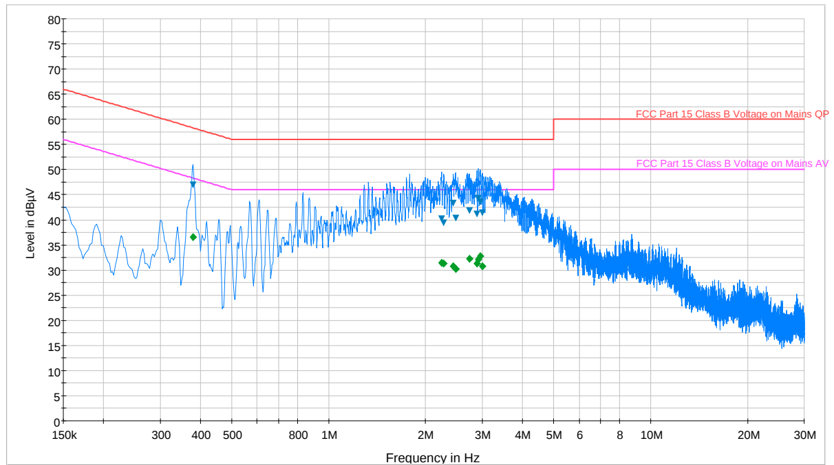
Plot 6-24. Line Conducted Plot with Bluetooth (L1)
