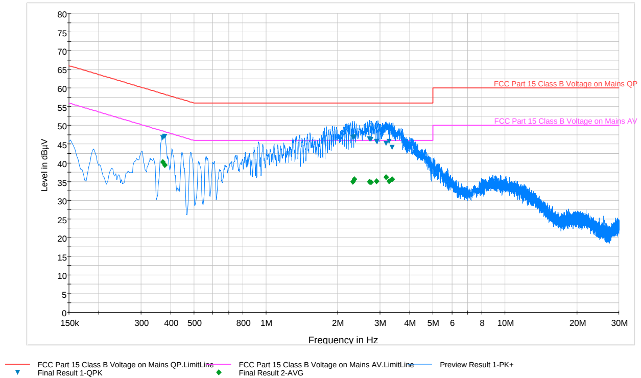
Plot 6-25. Line Conducted Plot with Bluetooth (N)
