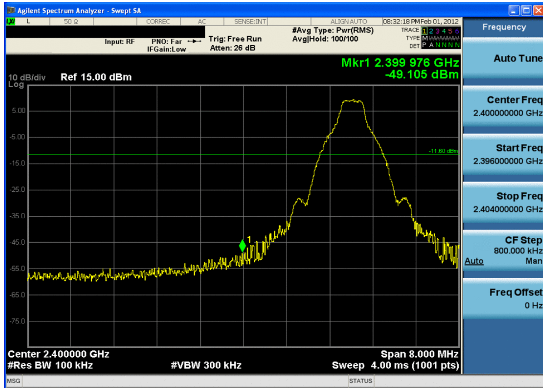
Plot 6-10. Band Edge Plot (Bluetooth with Hopping Disabled, 3Mbps – Ch. 0)
