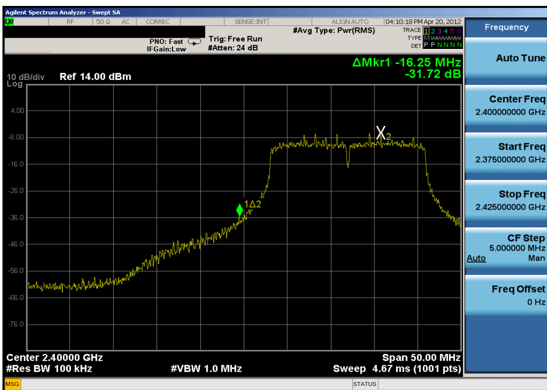
Plot 6-23. Band Edge Plot (802.11n – Ch. 1)
