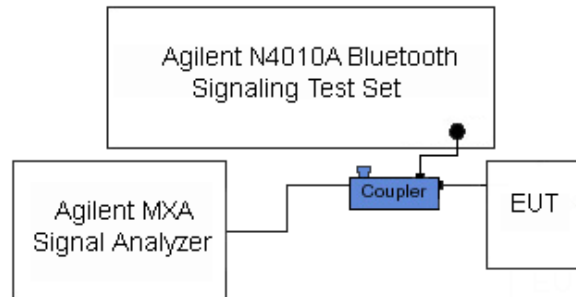
Figure 6-2. Test Instrument & Measurement Setup
