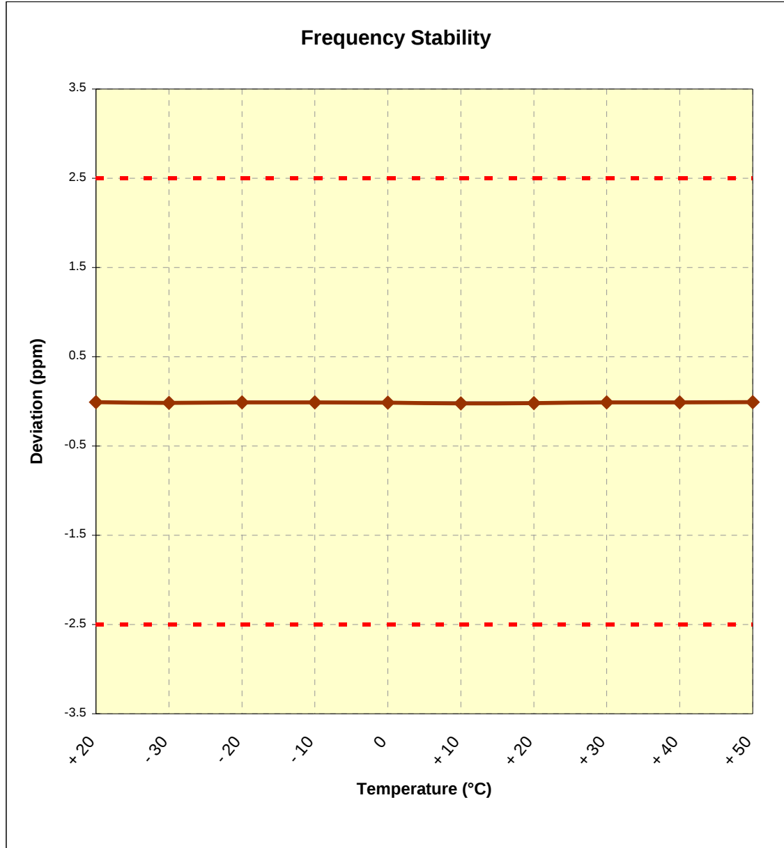
Figure 6-1. Frequency Stability Graph (Cellular GSM Mode – Ch. 190)
