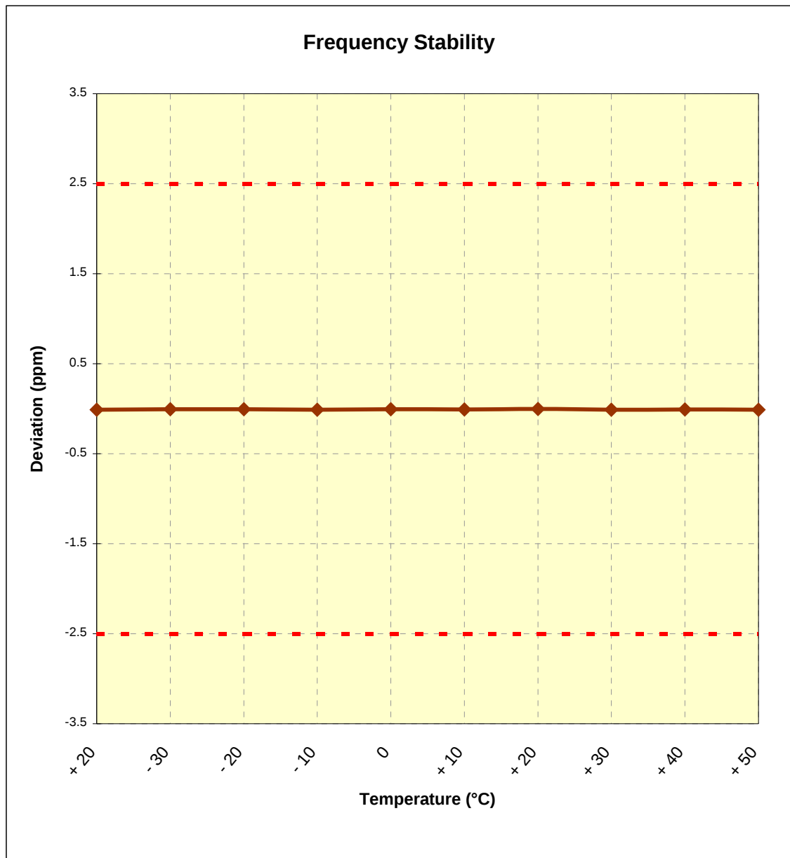
Figure 6-2. Frequency Stability Graph (PCS GSM Mode – Ch. 661)
