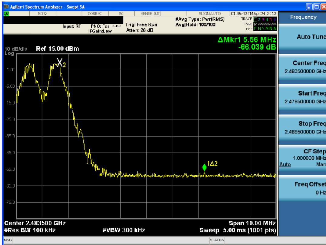
Plot 6-13. Band Edge Plot (Bluetooth with Hopping Enabled, 1Mbps – Ch. 78)
