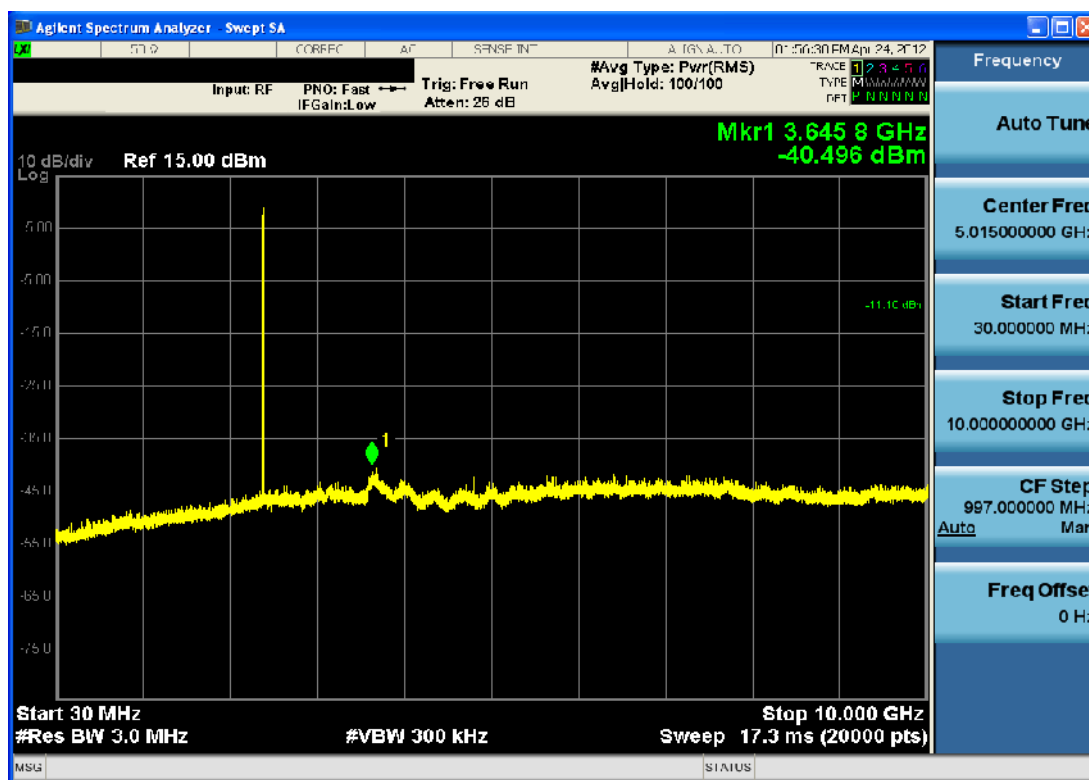
Plot 6-18. Conducted Spurious Plot (Bluetooth, 1Mbps – Ch. 0)
