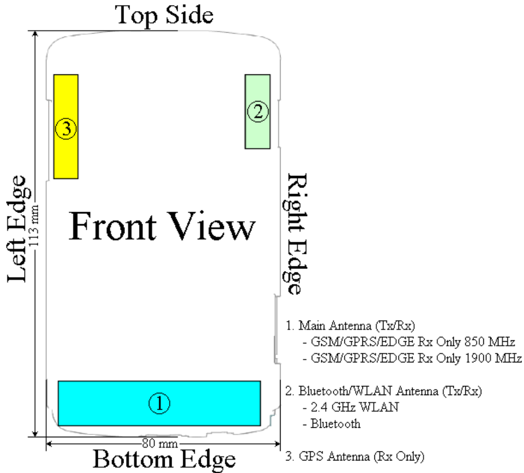
Figure 1-1 DUT Antenna Locations
