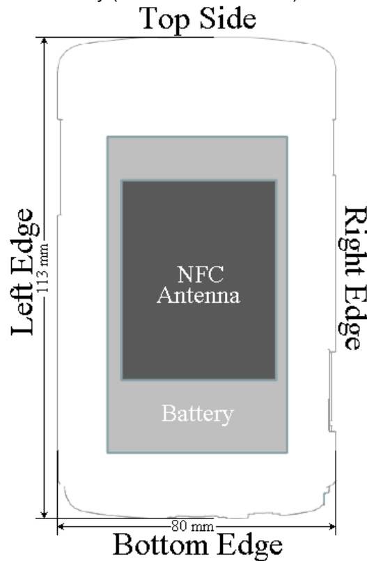
Figure 1-2 NFC Antenna Locations
