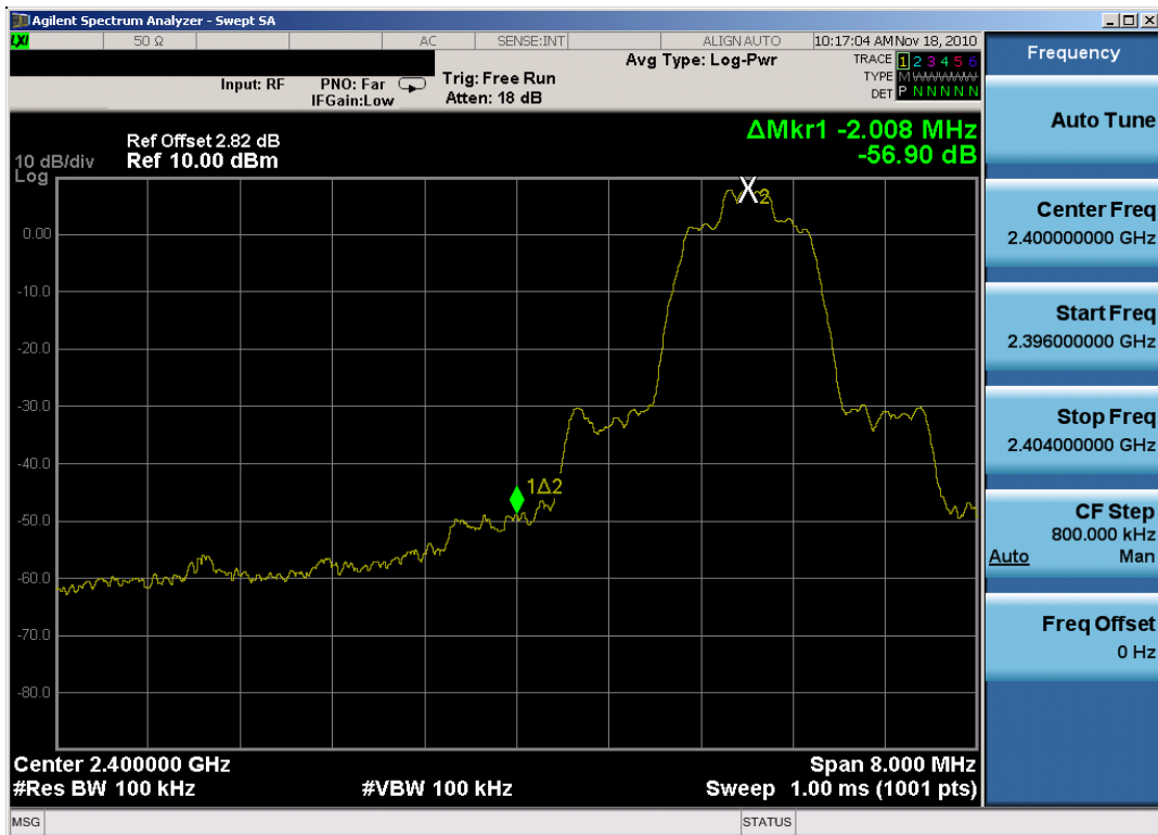
Plot 6-14. Band Edge Plot (Bluetooth, 2Mbps – Ch. 0)
