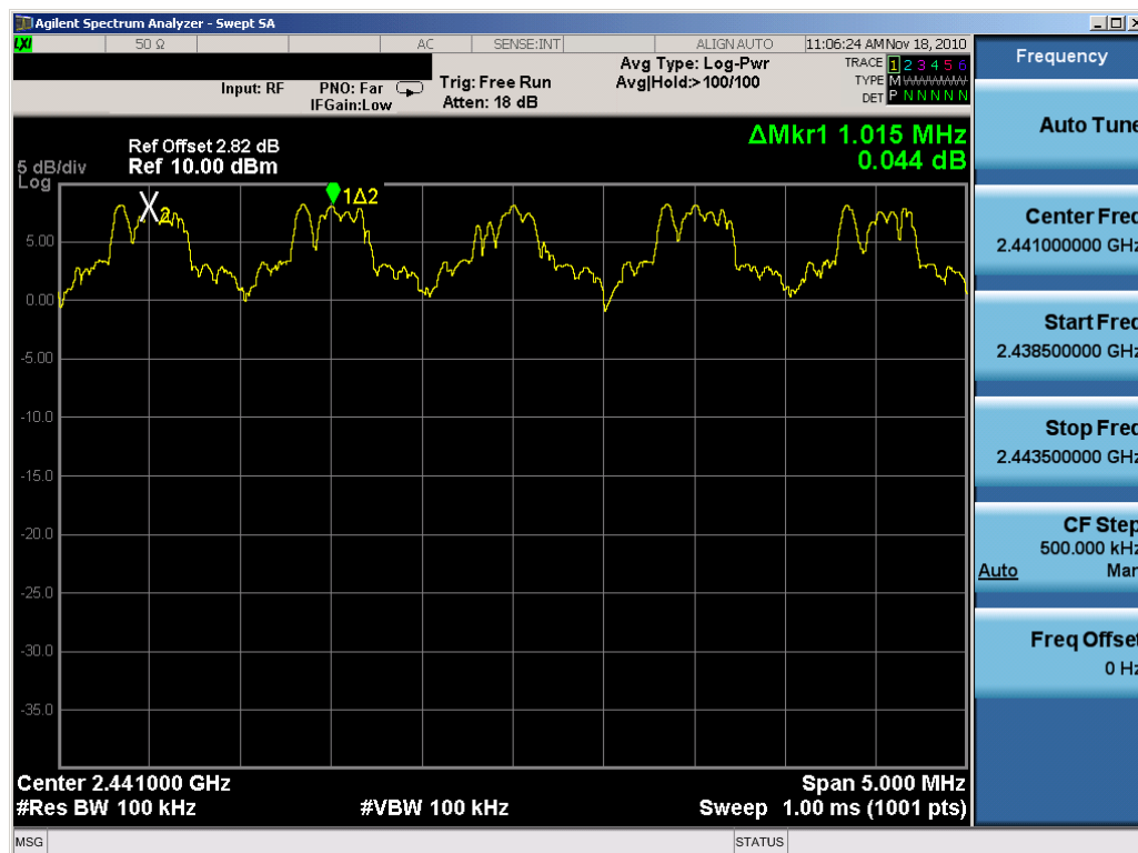
Plot 6-16. Channel Spacing Plot (Bluetooth)
