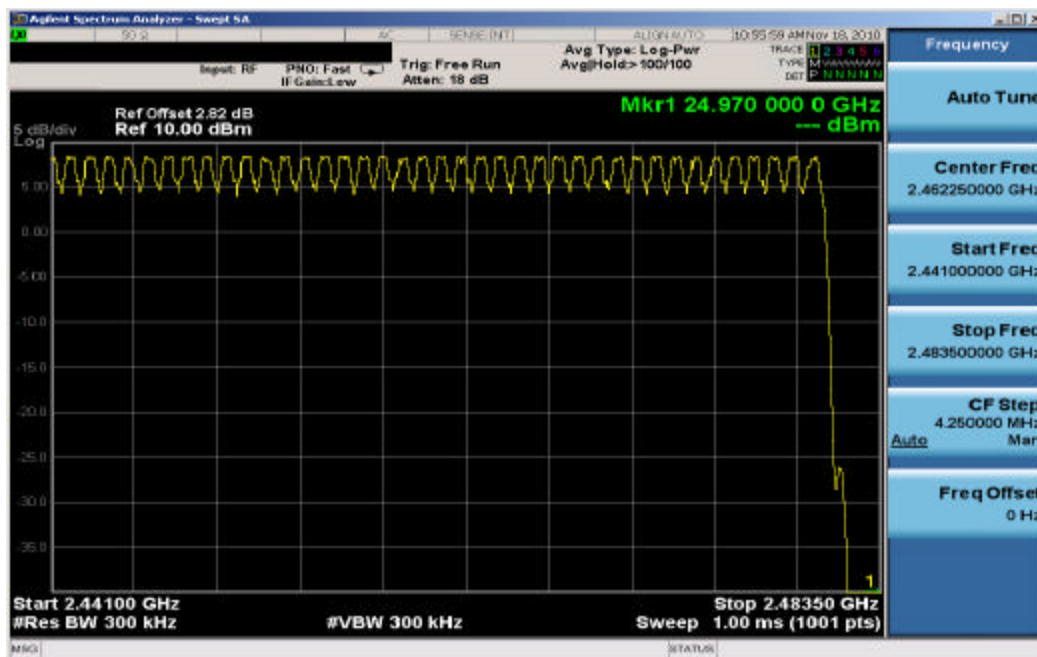
Plot 6-19. High End Spectrum Channel Hopping Plot (Bluetooth)
