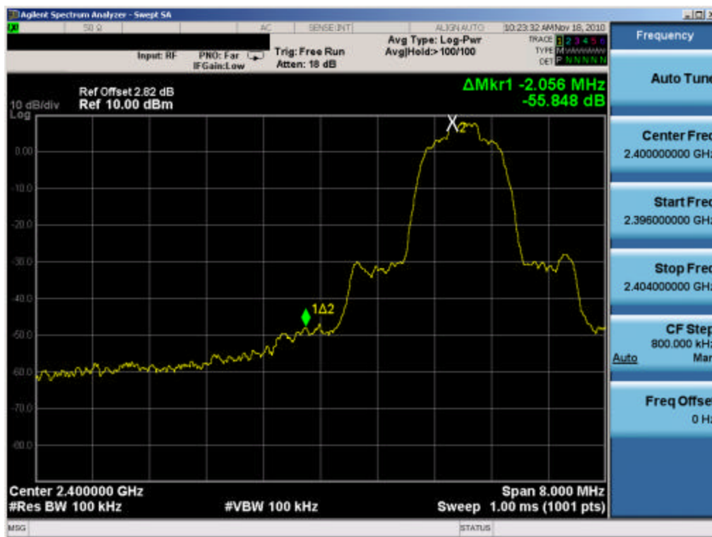
Plot 6-10. Band Edge Plot (Bluetooth, 3Mbps – Ch. 0)
