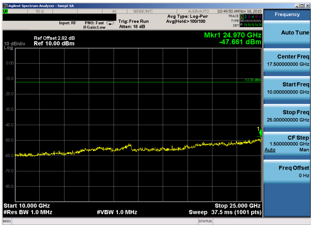
Plot 6-25. Conducted Spurious Plot (Bluetooth, 3Mbps – Ch. 78)
