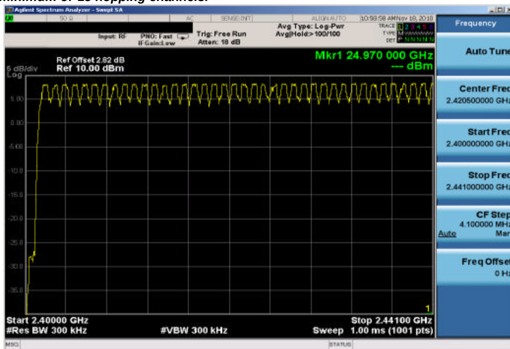
Plot 6-18. Low End Spectrum Channel Hopping Plot (Bluetooth)
