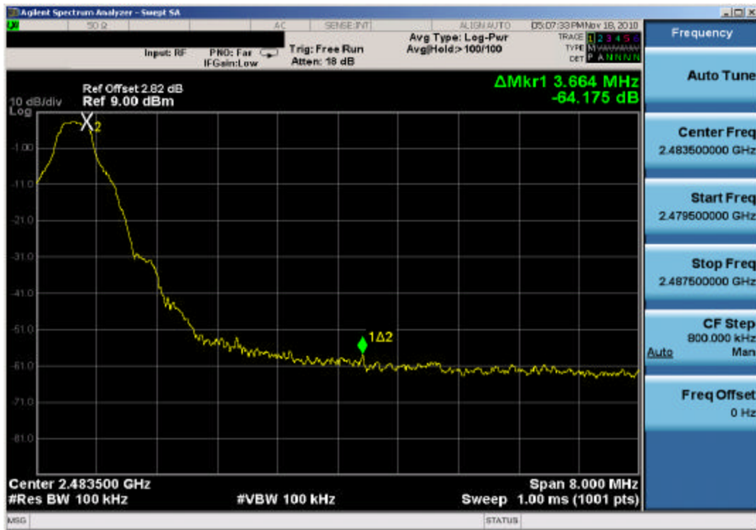
Plot 6-13. Band Edge Plot (Bluetooth, 1Mbps – Ch. 78)
