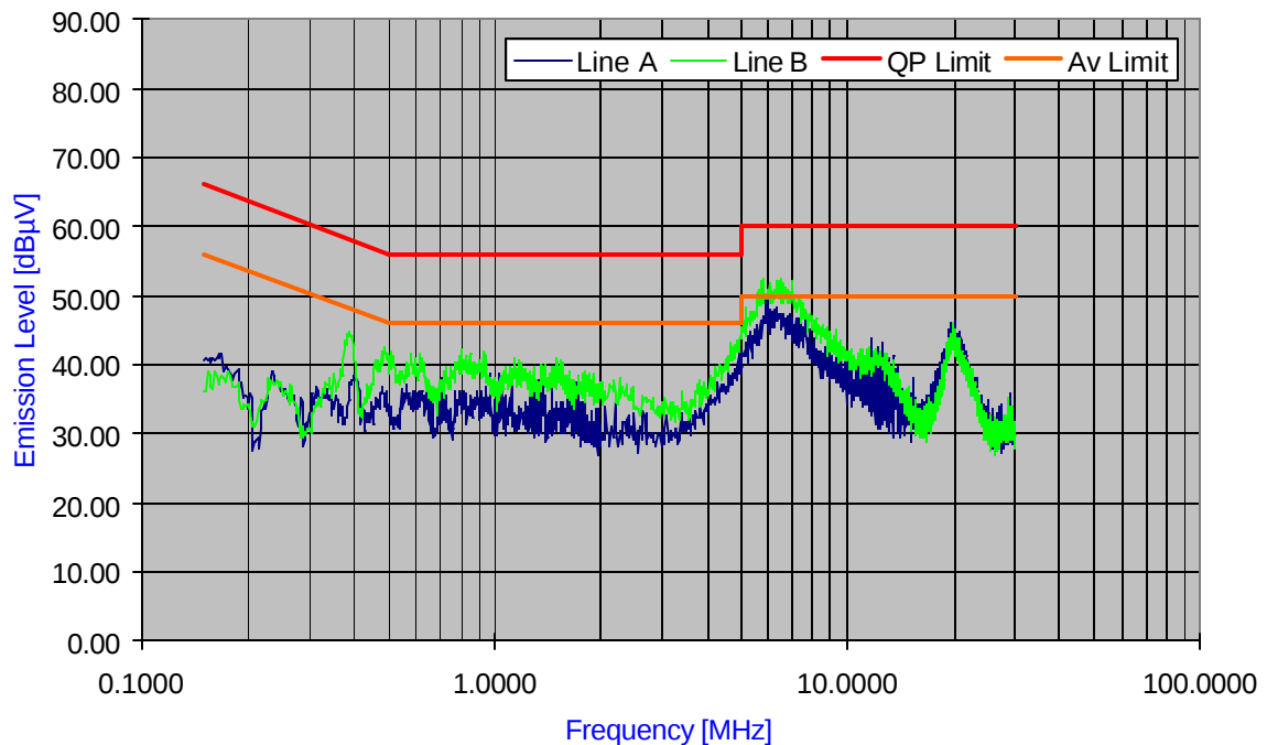
Plot 6-26. Line Conducted Plot with Bluetooth
