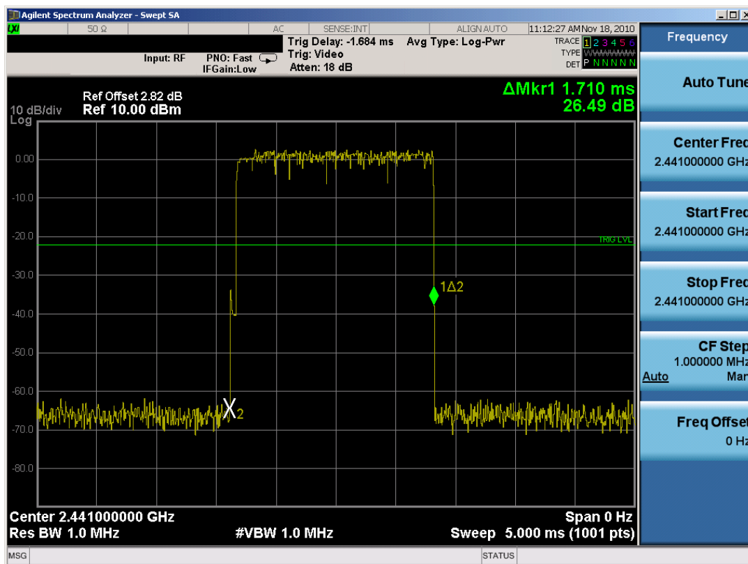
Plot 6-17. Time of Occupancy Plot (Bluetooth)
