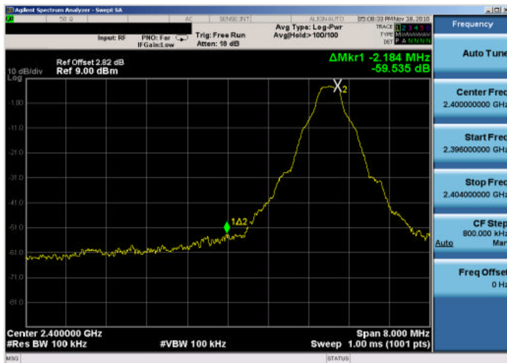
Plot 6-12. Band Edge Plot (Bluetooth, 1Mbps - Ch. 0)
