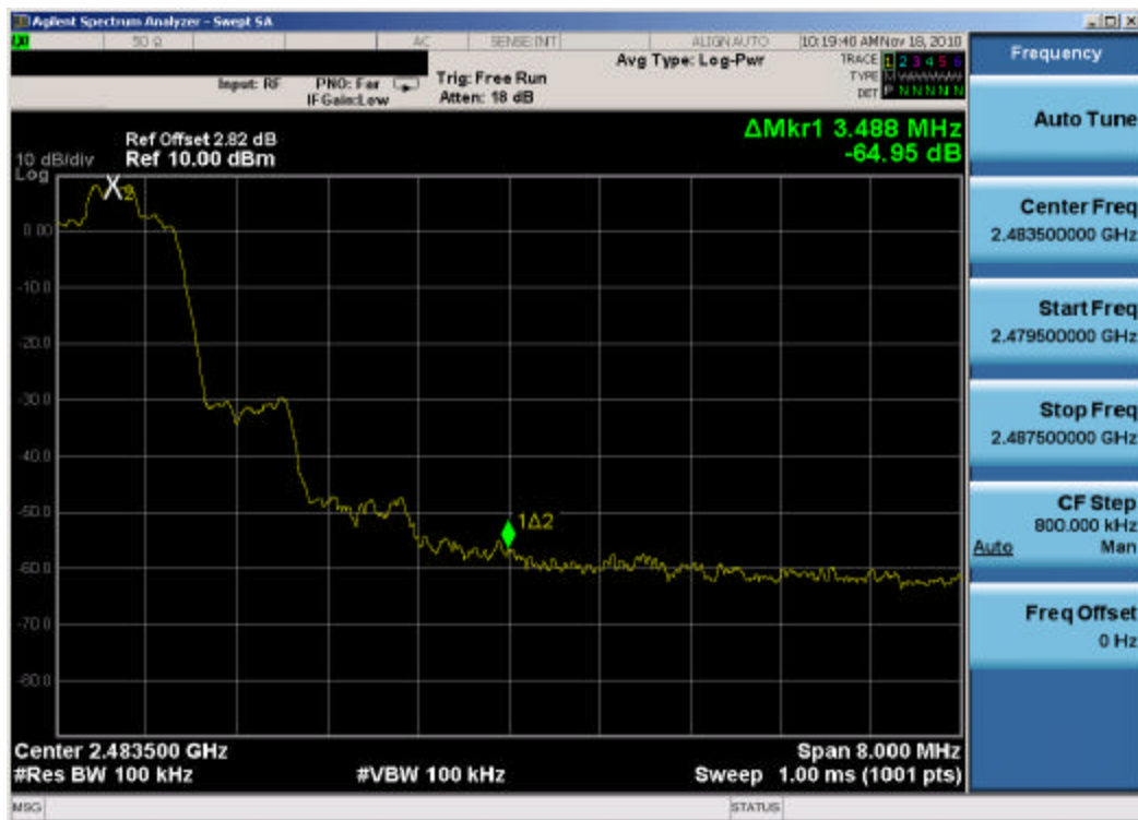
Plot 6-15. Band Edge Plot (Bluetooth, 2Mbps – Ch. 78)
