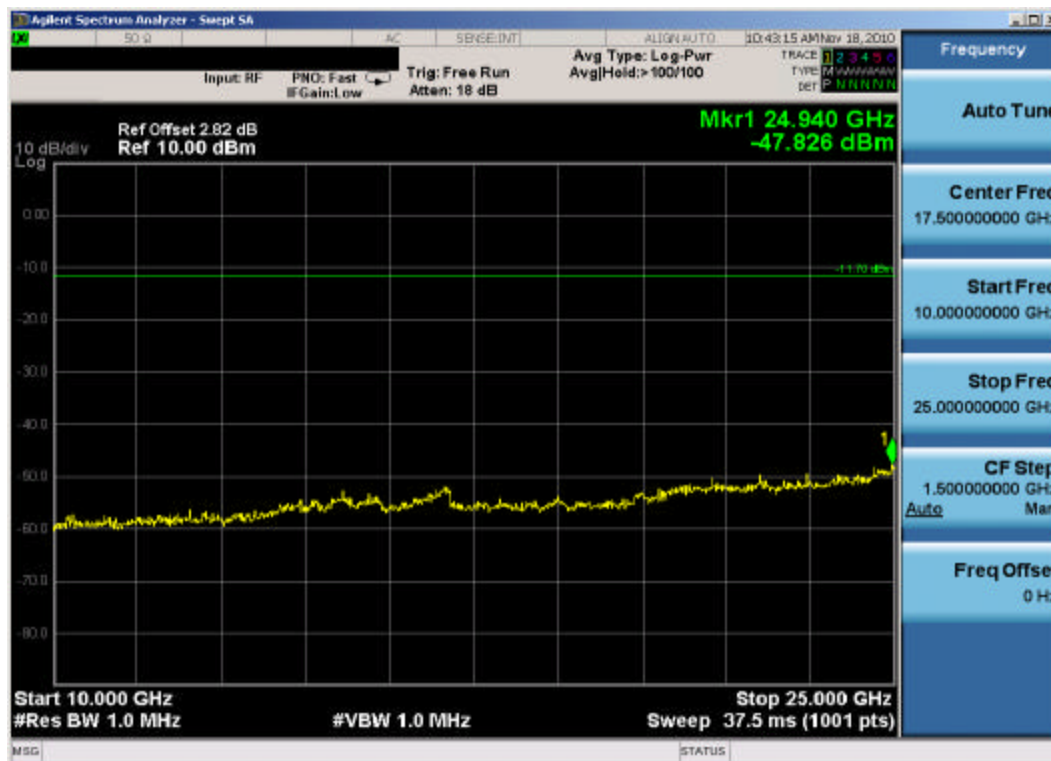
Plot 6-23. Conducted Spurious Plot (Bluetooth, 3Mbps – Ch. 39)
