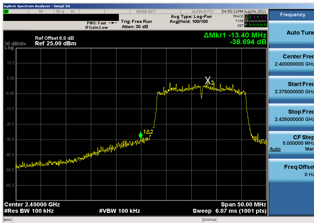
Plot 6-23. Band Edge Plot (802.11n – Ch. 1)
