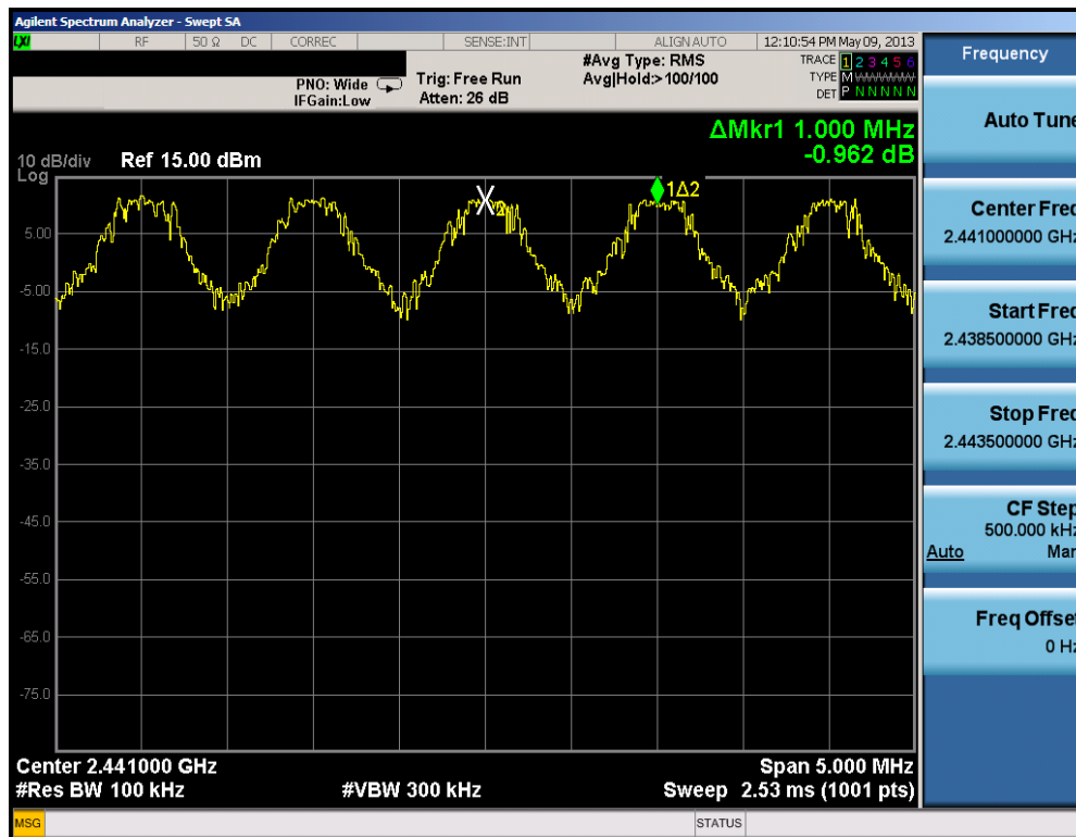
Plot 6-32. Channel Spacing Plot (Bluetooth)
