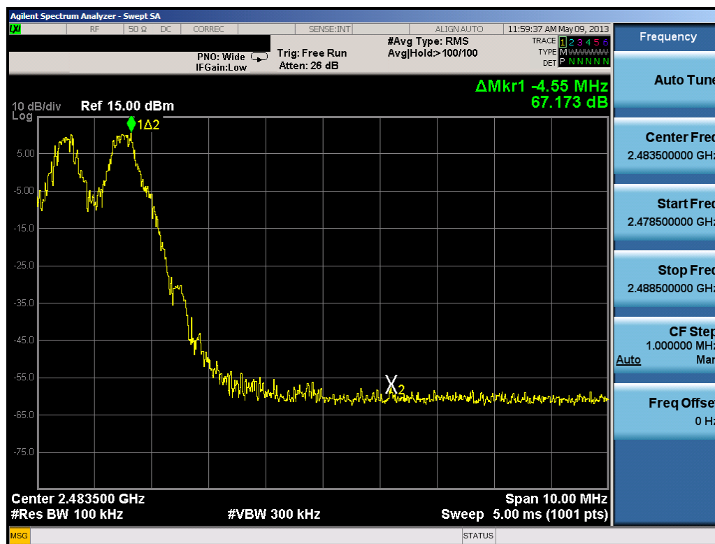
Plot 6-31. Band Edge Plot (Bluetooth with Hopping Enabled, 1Mbps)
