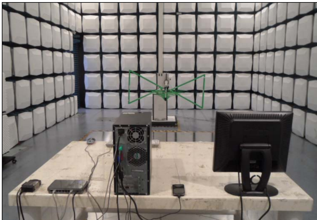
[ Radiated Disturbance for Below 1 GHz – Rear ]
