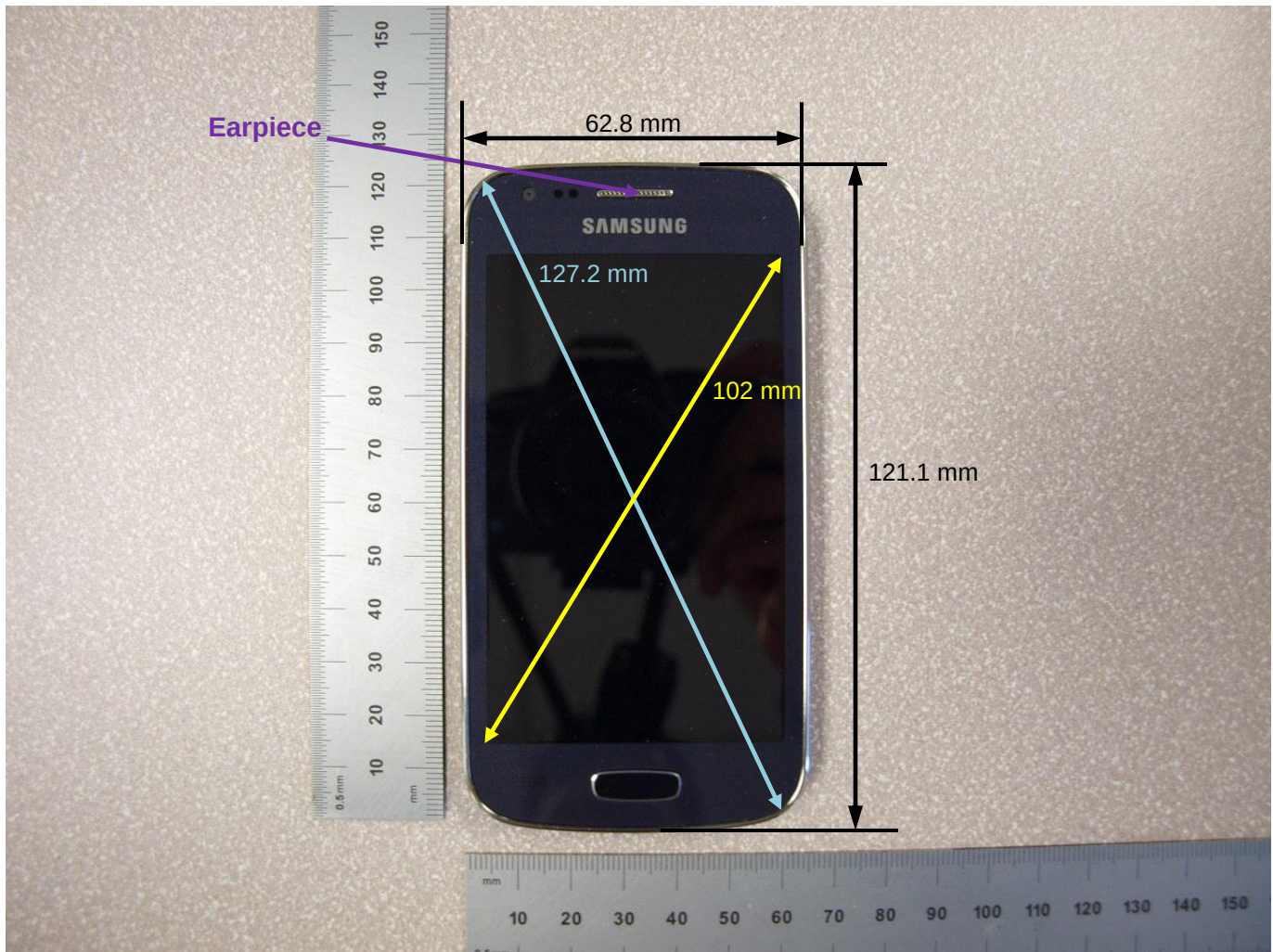
Overall Dimensions
