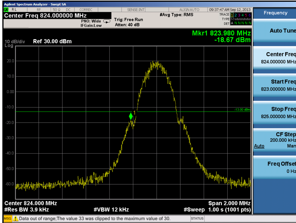
Plot 6-27. Band Edge Plot (Cellular GSM Mode – Ch. 128)
