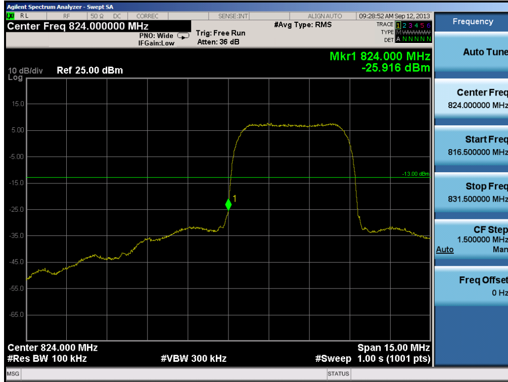
Plot 6-31. Band Edge Plot (Cellular WCDMA Mode – Ch. 4132)
