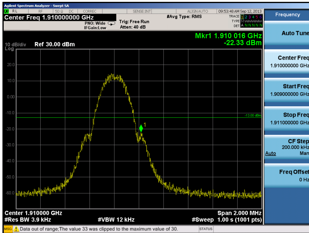
Plot 6-30. Band Edge Plot (PCS GSM Mode – Ch. 810)
