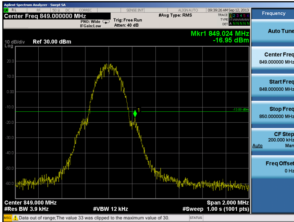
Plot 6-28. Band Edge Plot (Cellular GSM Mode – Ch. 251)
