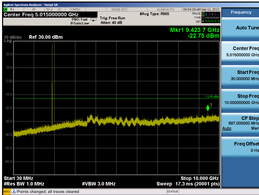
Plot 6-19. Conducted Spurious Plot (PCS GSM Mode – Ch. 810)
