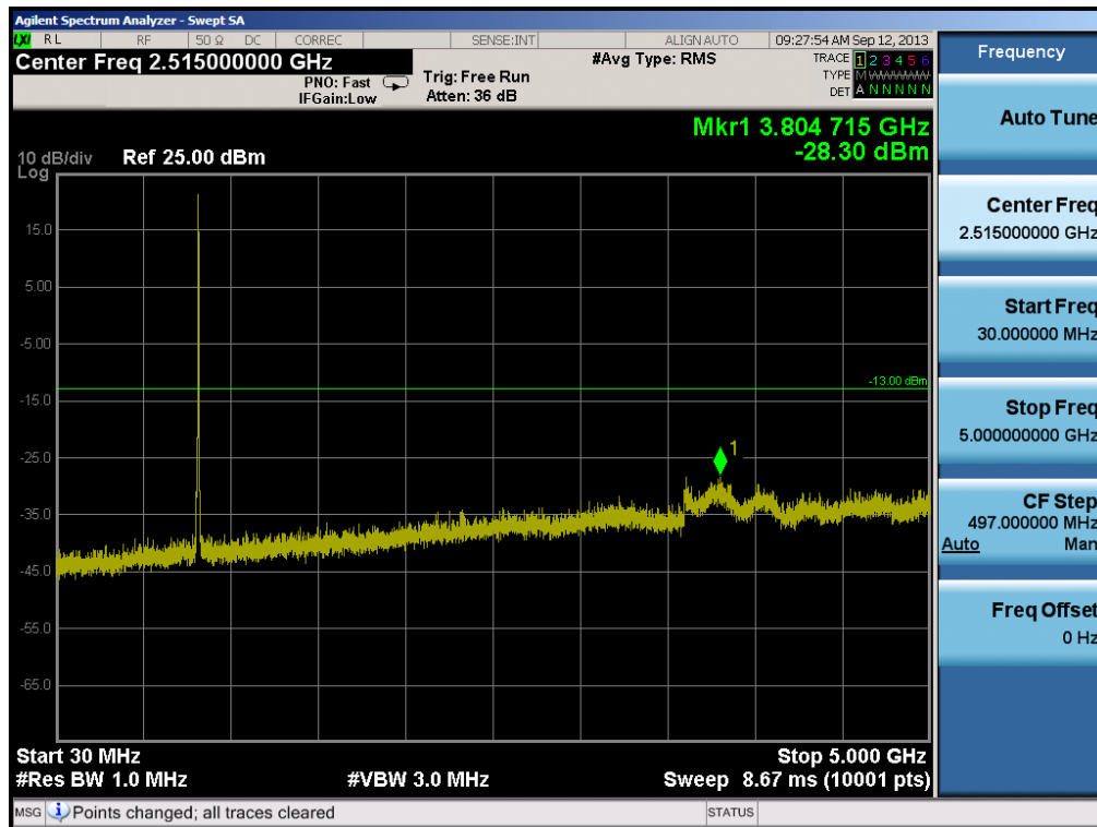
Plot 6-23. Conducted Spurious Plot (Cellular WCDMA Mode – Ch. 4183)
