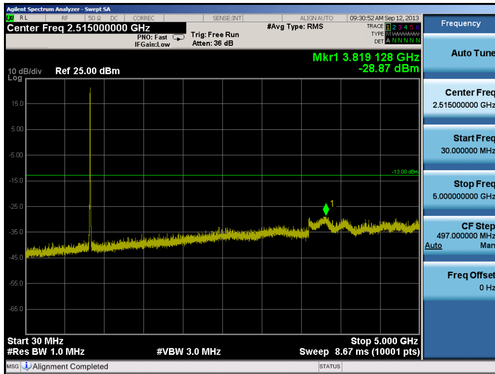
Plot 6-25. Conducted Spurious Plot (Cellular WCDMA Mode – Ch. 4233)
