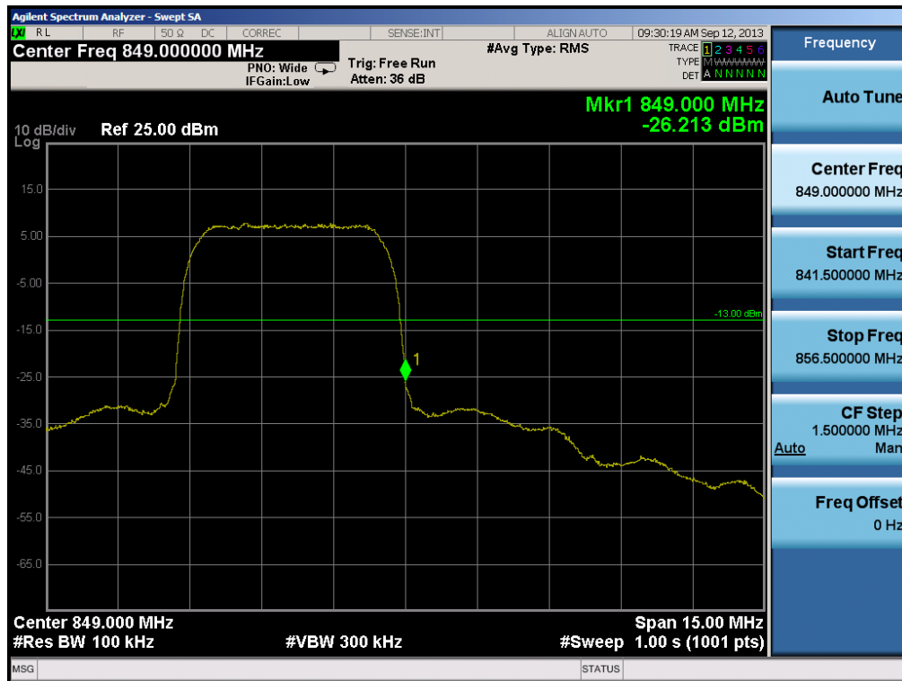
Plot 6-32. Band Edge Plot (Cellular WCDMA Mode – Ch. 4233)
