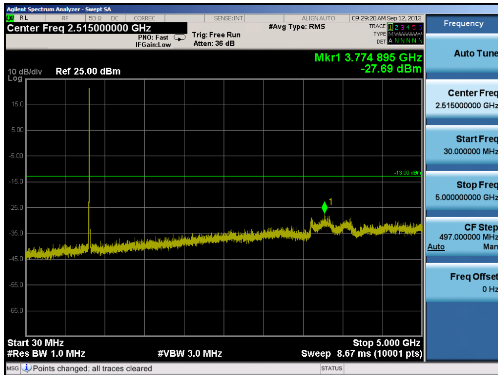
Plot 6-21. Conducted Spurious Plot (Cellular WCDMA Mode – Ch. 4132)
