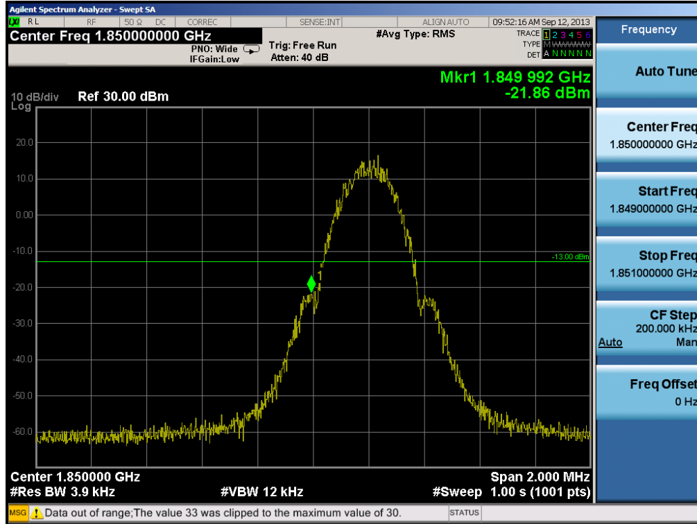
Plot 6-29. Band Edge Plot (PCS GSM Mode – Ch. 512)
