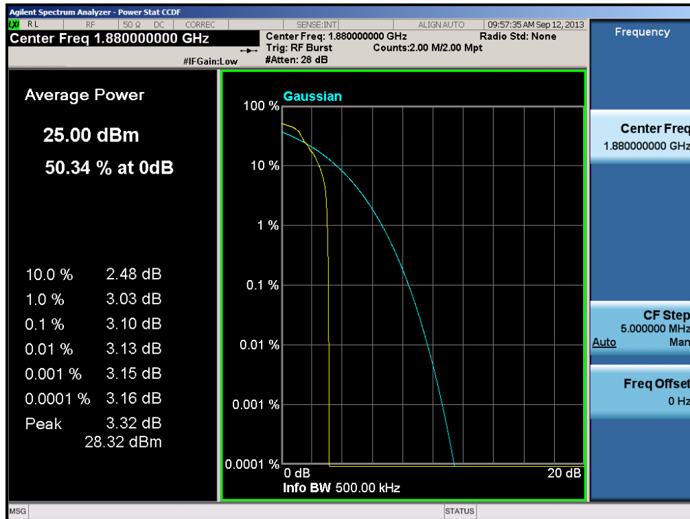
Plot 6-34. Peak-Average Ratio Plot (EDGE1900 Mode – Ch. 661)
