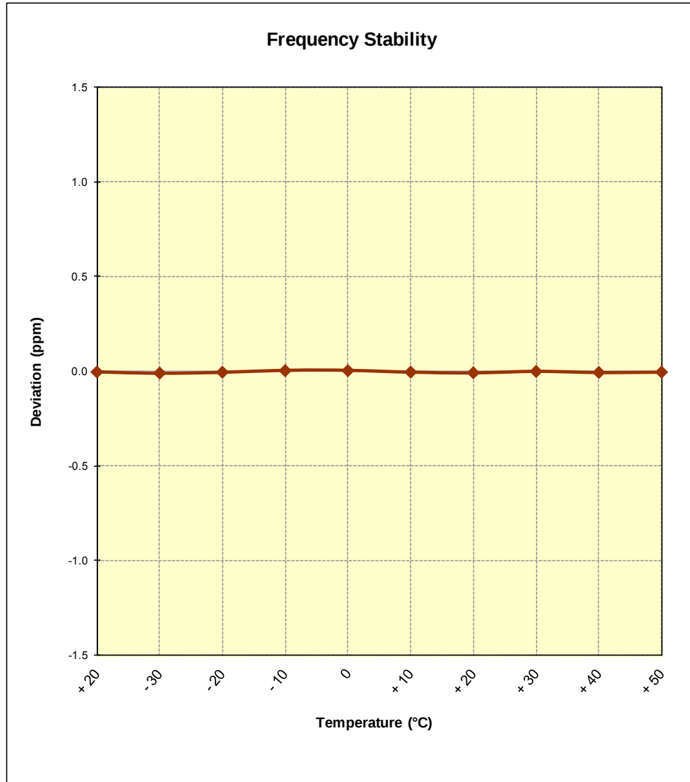
Figure 6-9. Frequency Stability Graph (PCS WCDMA Mode – Ch. 9400)
