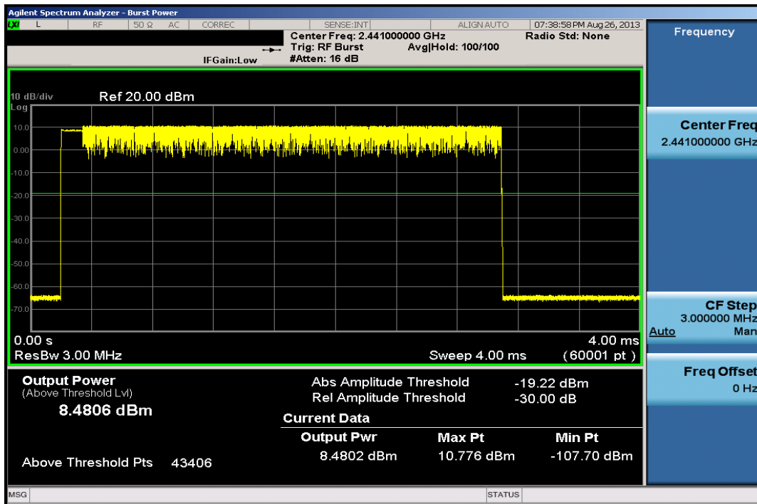
Plot 6-23. Average Conducted Power (2Mbps – Ch. 39)
