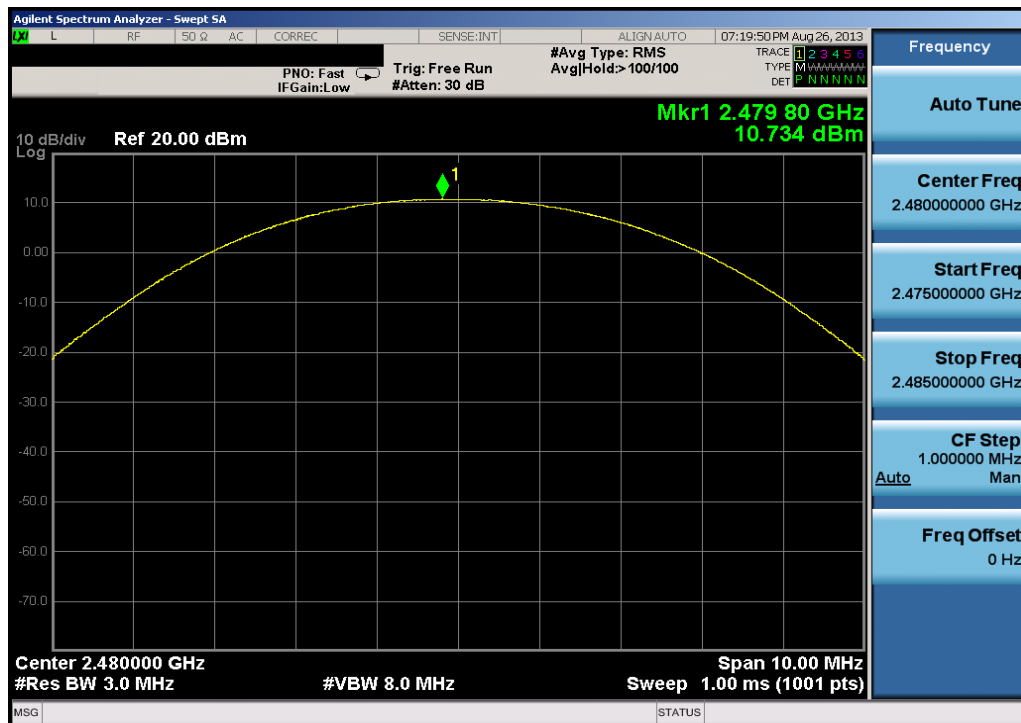
Plot 6-15. Peak Conducted Power (2Mbps – Ch. 78)
