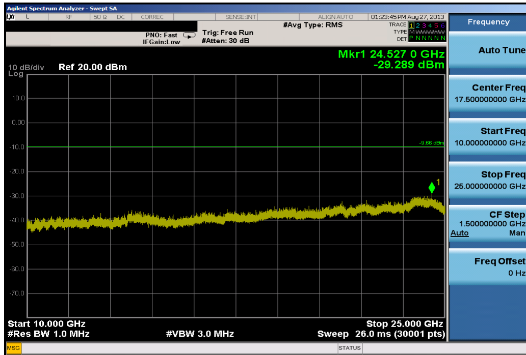
Plot 6-41. Conducted Spurious Plot (Bluetooth, 3Mbps – Ch. 78)
