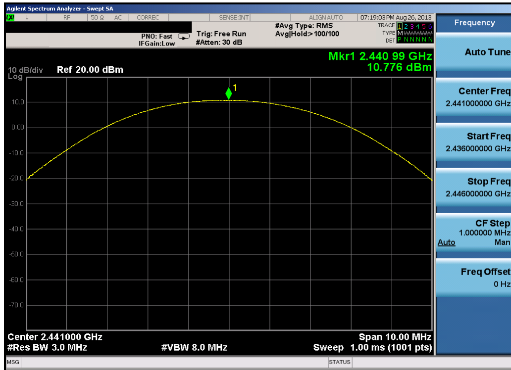
Plot 6-14. Peak Conducted Power (2Mbps – Ch. 39)
