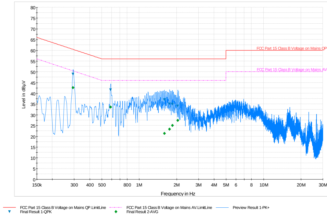
Plot 6-45. Line-Conducted Test Plot (N)
