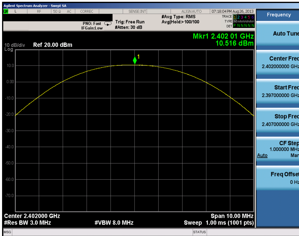
Plot 6-13. Peak Conducted Power (2Mbps – Ch. 0)
