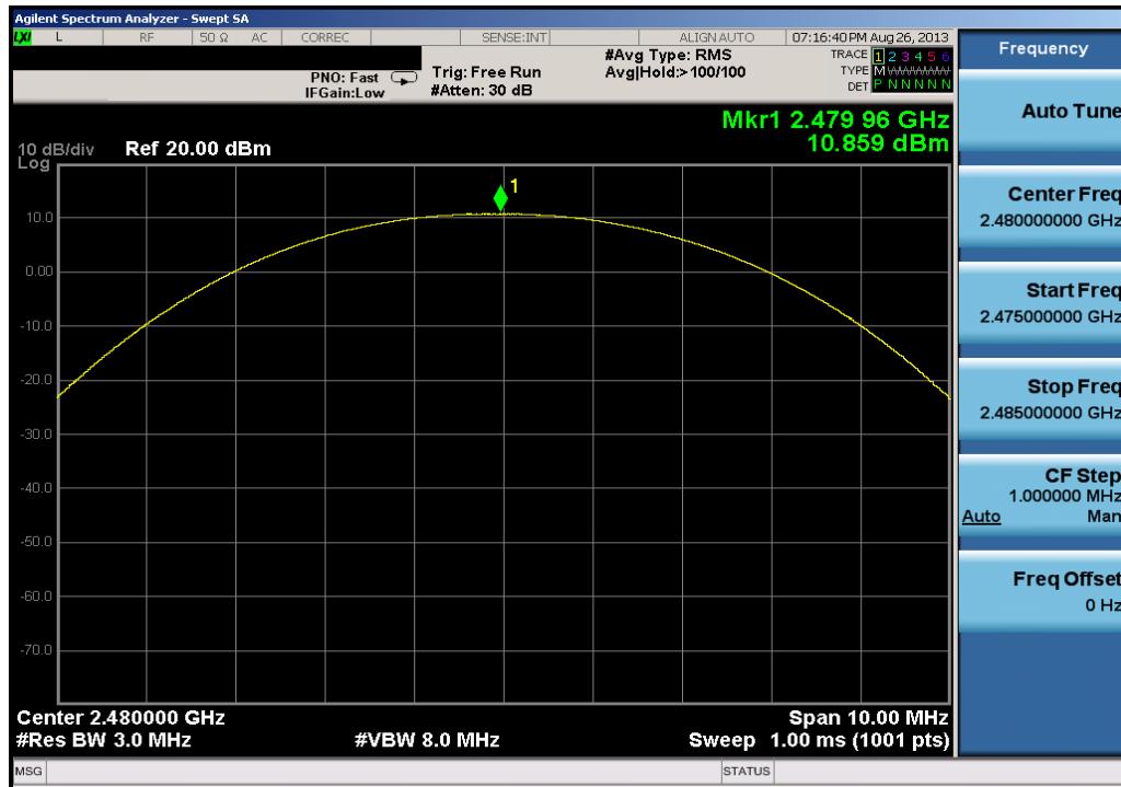
Plot 6-12. Peak Conducted Power (1Mbps – Ch. 78)
