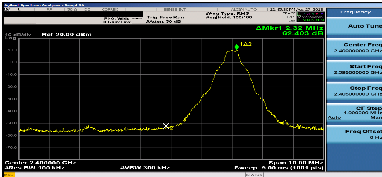
Plot 6-28. Band Edge Plot (Bluetooth with Hopping Disabled, 3Mbps – Ch. 0)
