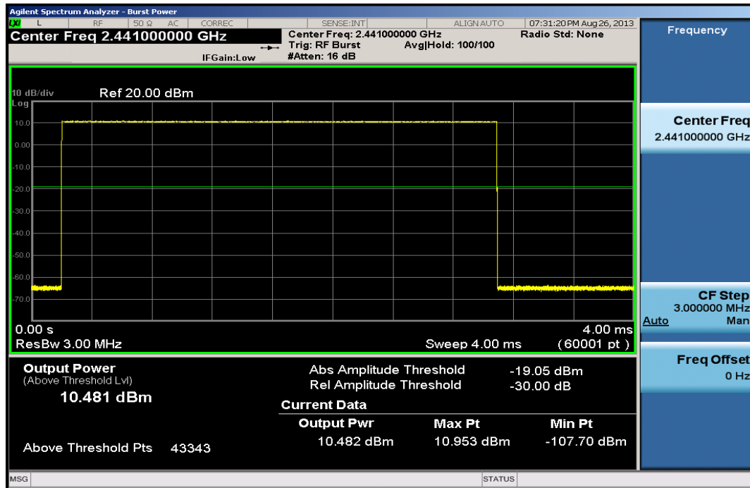
Plot 6-20. Average Conducted Power (1Mbps – Ch. 39)
