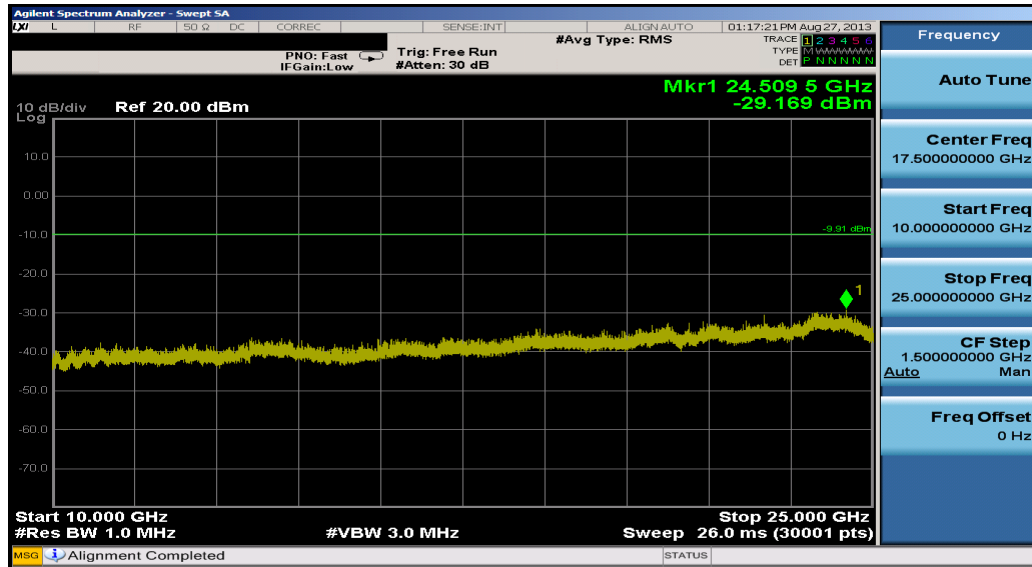
Plot 6-37. Conducted Spurious Plot (Bluetooth, 3Mbps – Ch. 0)
