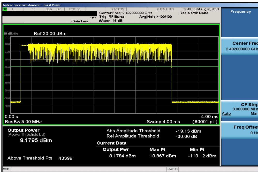
Plot 6-25. Average Conducted Power (3Mbps – Ch. 0)
