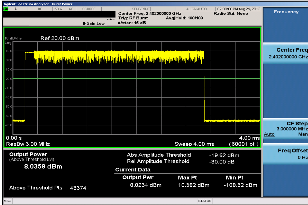
Plot 6-22. Average Conducted Power (2Mbps – Ch. 0)
