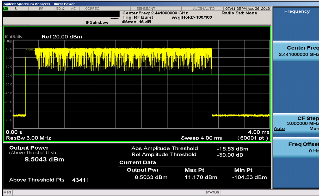
Plot 6-26. Average Conducted Power (3Mbps – Ch. 39)
