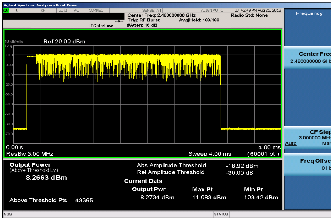
Plot 6-27. Average Conducted Power (3Mbps – Ch. 78)
