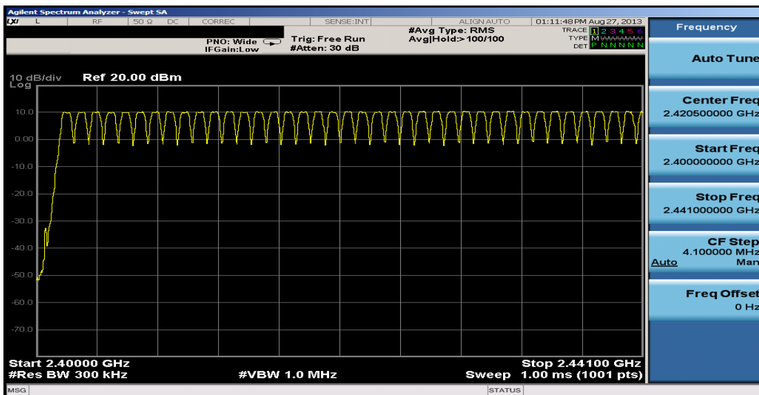
Plot 6-34. Low End Spectrum Channel Hopping Plot (Bluetooth)
