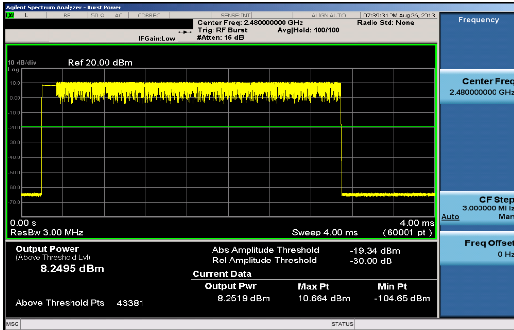
Plot 6-24. Average Conducted Power (2Mbps – Ch. 78)
