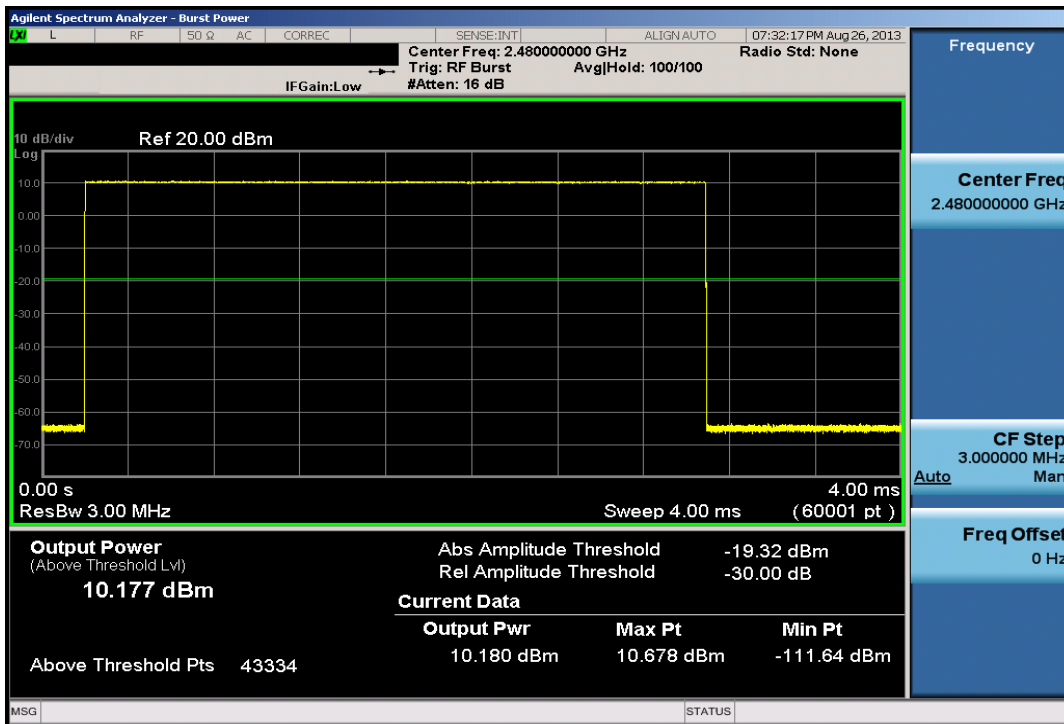
Plot 6-21. Average Conducted Power (1Mbps – Ch. 78)
