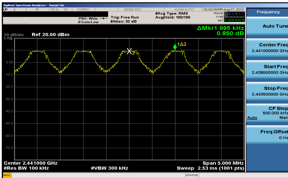
Plot 6-32. Channel Spacing Plot (Bluetooth)
