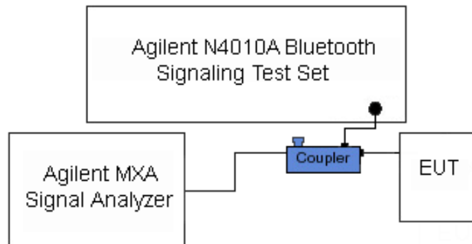
Figure 6-1. Test Instrument & Measurement Setup
