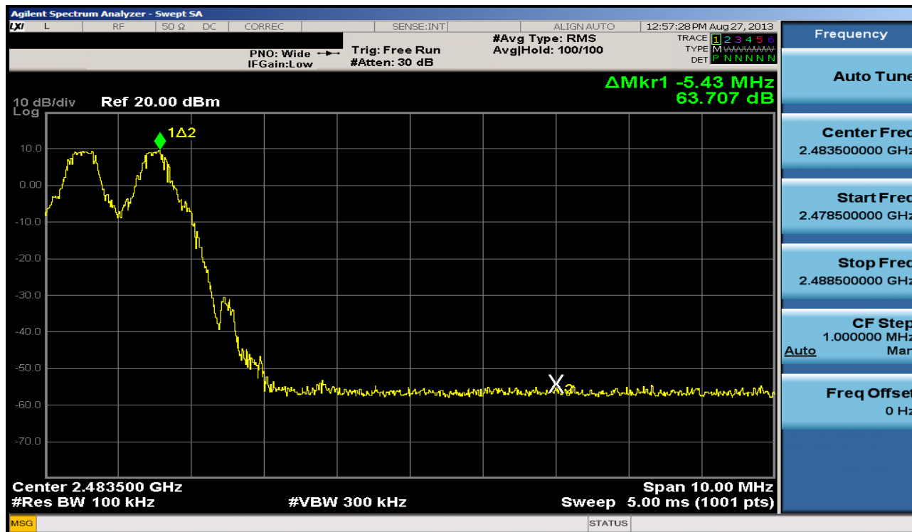
Plot 6-31. Band Edge Plot (Bluetooth with Hopping Enabled, 3Mbps)
