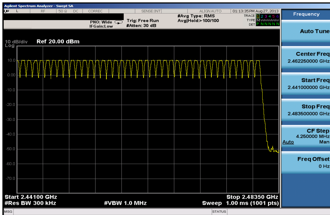
Plot 6-35. High End Spectrum Channel Hopping Plot (Bluetooth)
