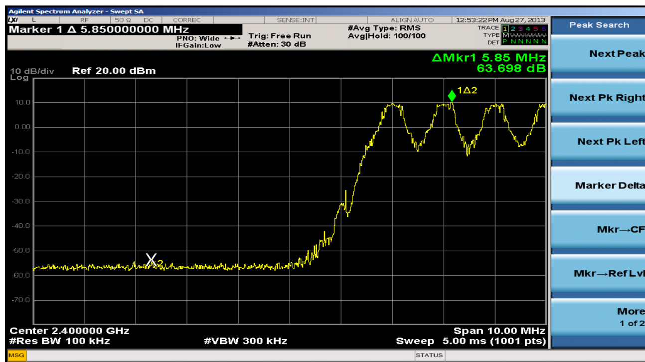
Plot 6-30. Band Edge Plot (Bluetooth with Hopping Enabled, 3Mbps)
