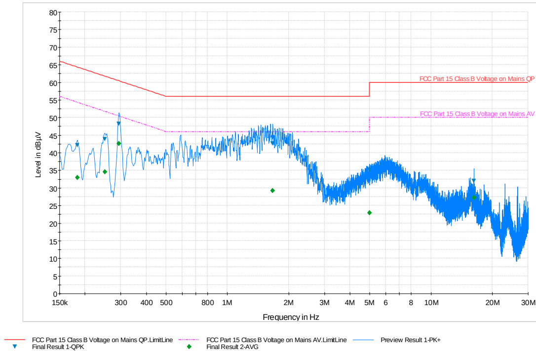
Plot 6-44. Line-Conducted Test Plot (L1)
