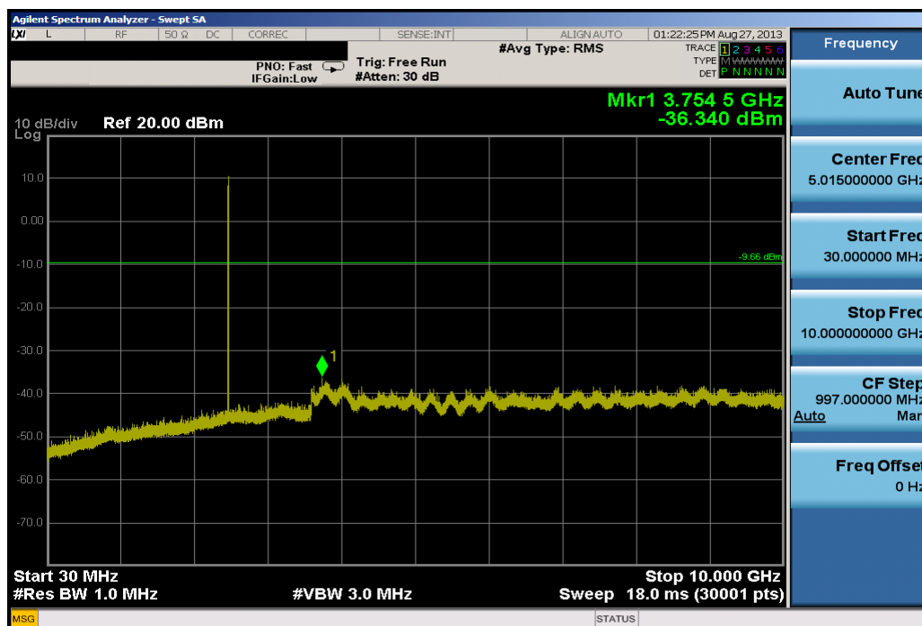
Plot 6-40. Conducted Spurious Plot (Bluetooth, 3Mbps – Ch. 78)
