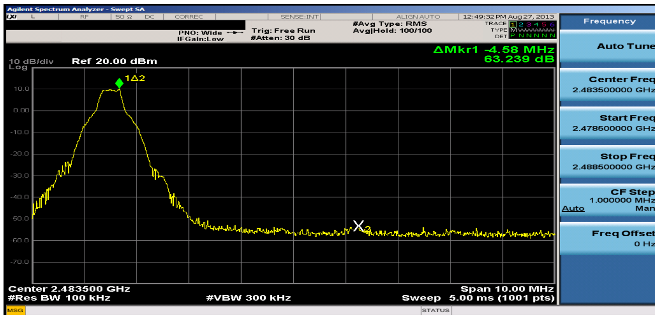
Plot 6-29. Band Edge Plot (Bluetooth with Hopping Disabled, 3Mbps – Ch. 78)
