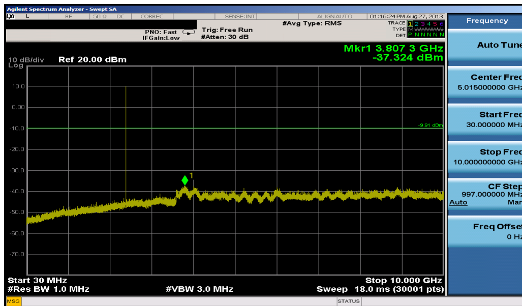
Plot 6-36. Conducted Spurious Plot (Bluetooth, 3Mbps – Ch. 0)
