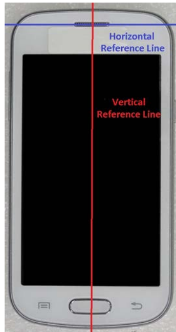
SAR Test Setup Photo 10 - Horizontal and Vertical Reference Lines
