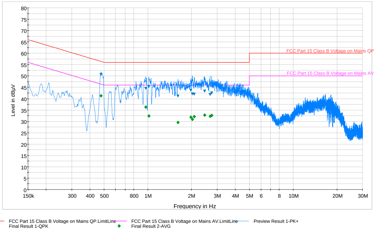
Plot 6-25. Line Conducted Plot with Bluetooth (N)
