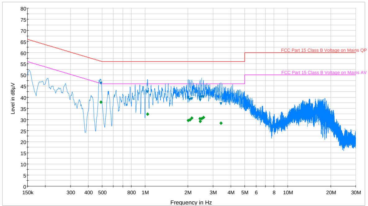
Plot 6-24. Line Conducted Plot with Bluetooth (L1)
