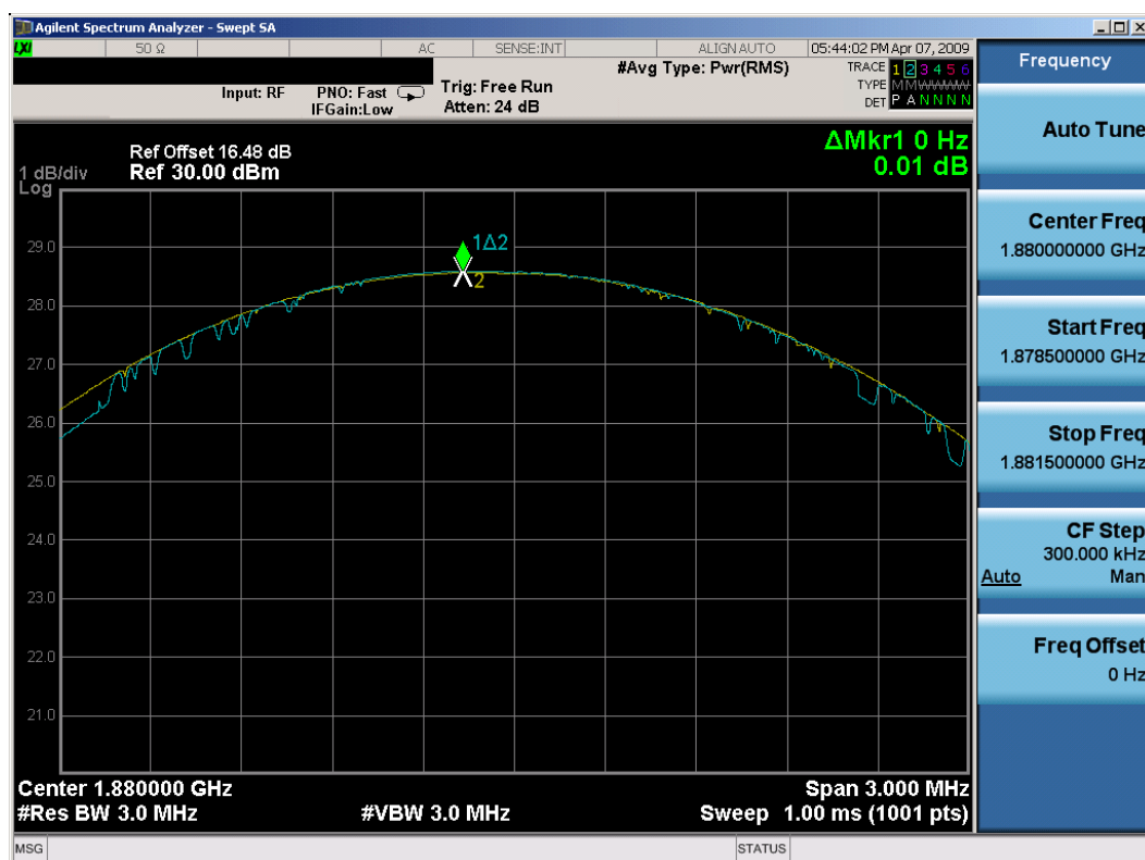
Plot 7-12. Peak-Average Ratio Plot (EDGE1900 – Ch. 661)
