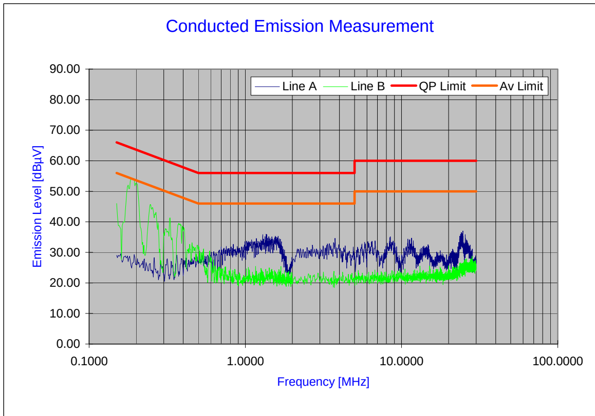
Plot 6-31. Line Conducted Plot with 802.11b
