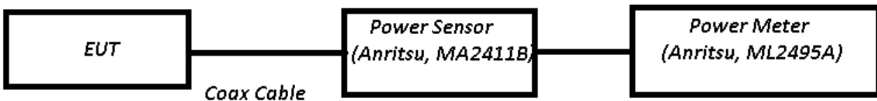
Figure 6-1. Test Instrument & Measurement Setup
