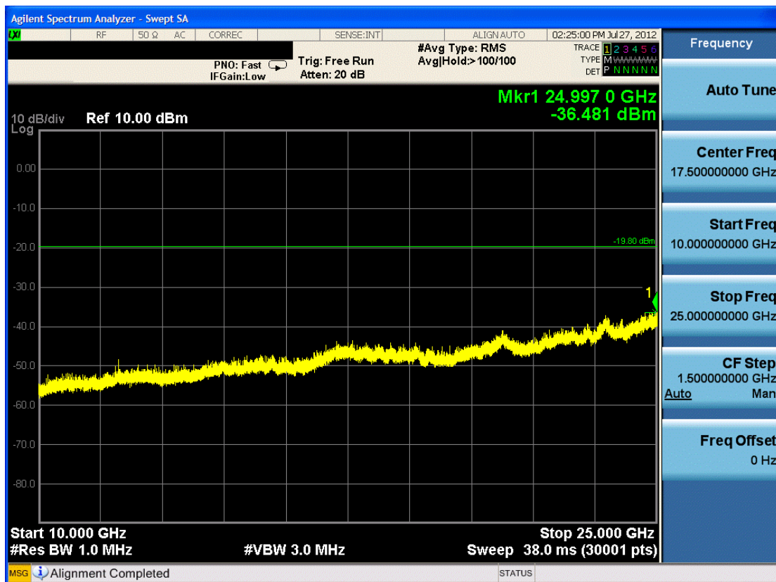
Plot 6-23. Conducted Spurious Plot (Bluetooth, 1Mbps – Ch. 78)
