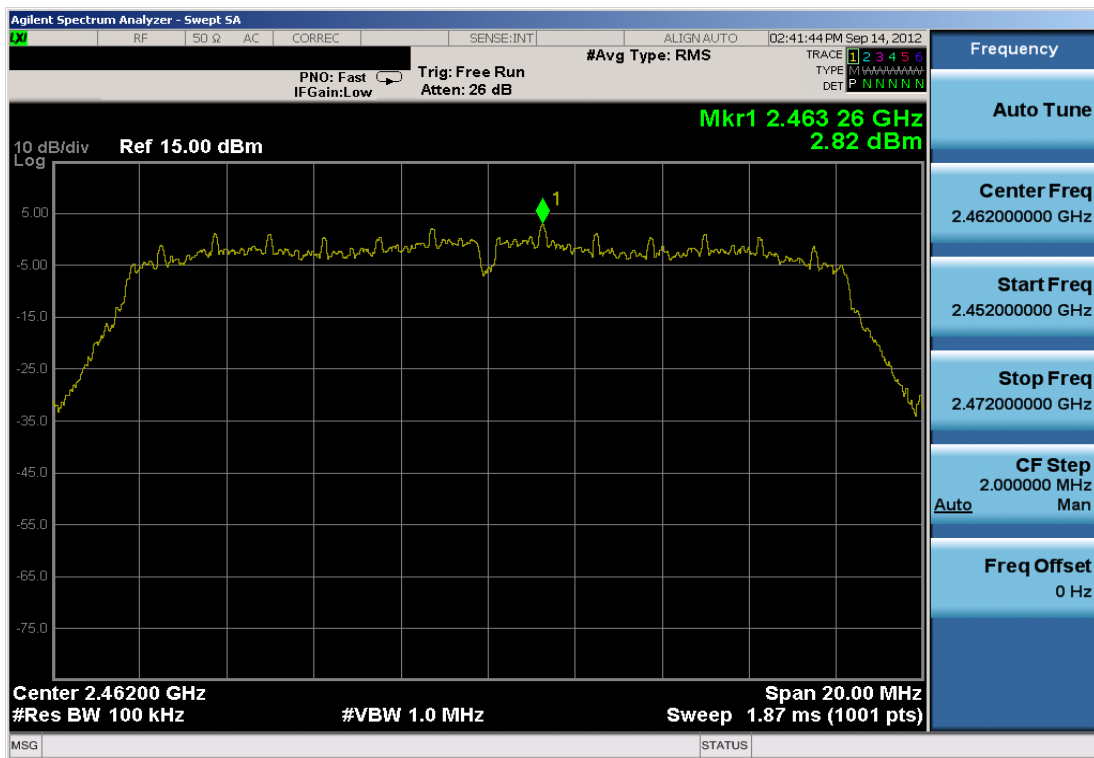
Plot 6-15. Power Spectral Density Plot (802.11g – Ch. 11)
