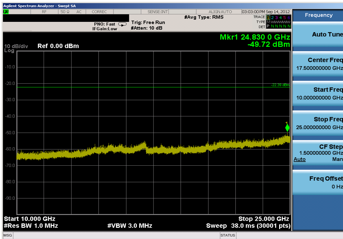
Plot 6-30. Conducted Spurious Plot (802.11b – Ch. 11)
