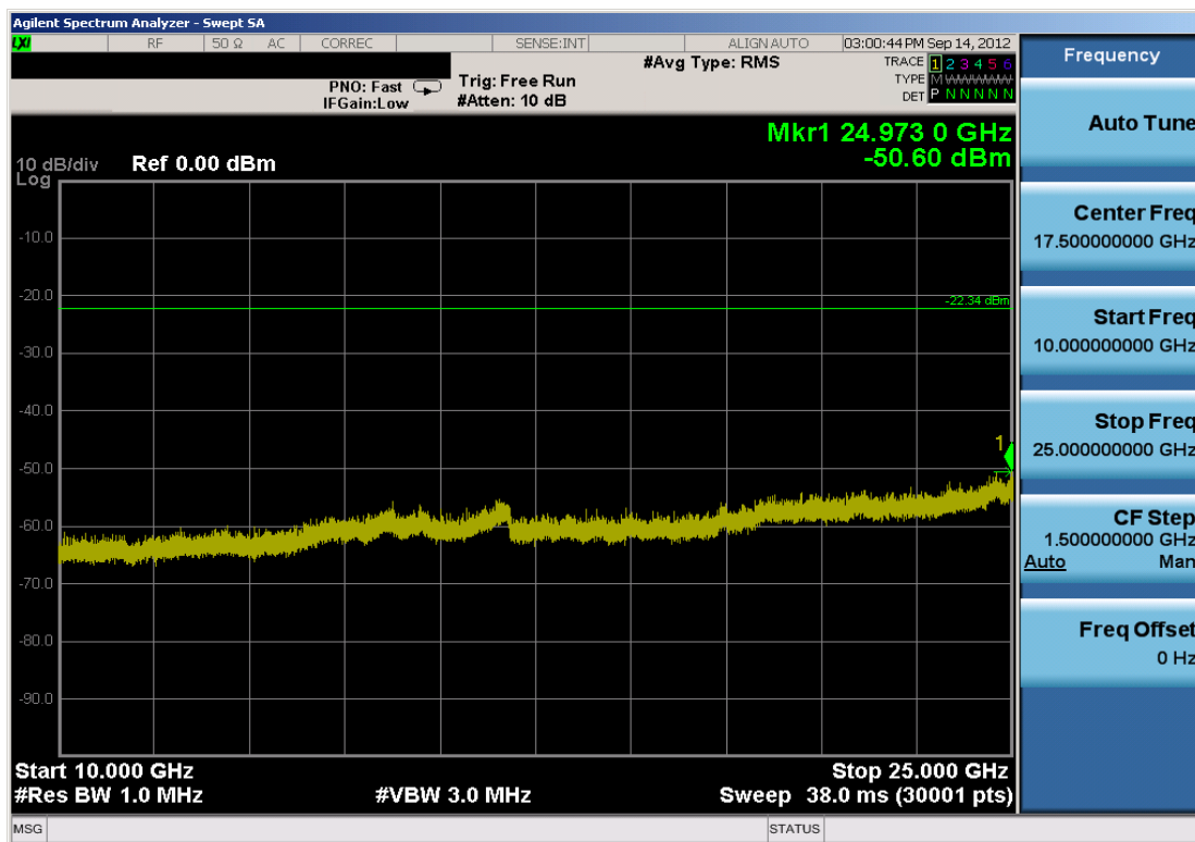
Plot 6-28. Conducted Spurious Plot (802.11b – Ch. 6)
