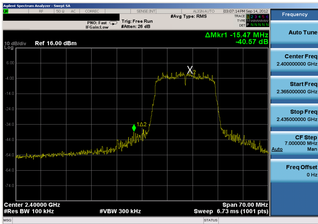
Plot 6-21. Band Edge Plot (802.11g – Ch. 1)
