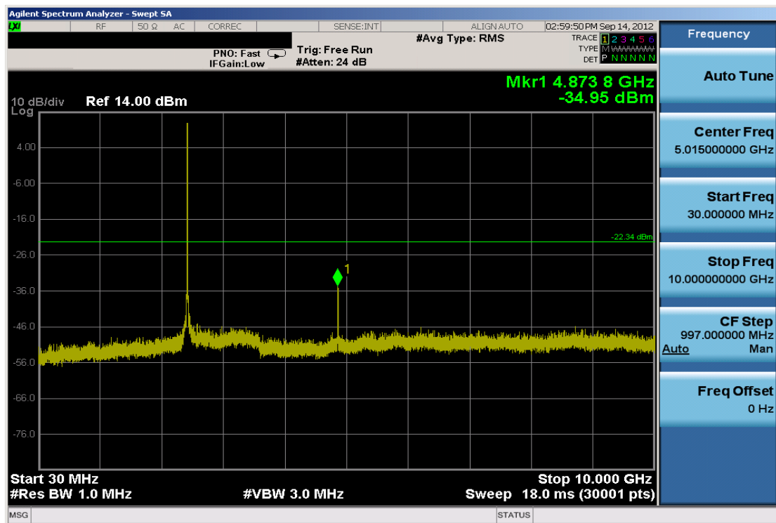
Plot 6-27. Conducted Spurious Plot (802.11b – Ch. 6)
