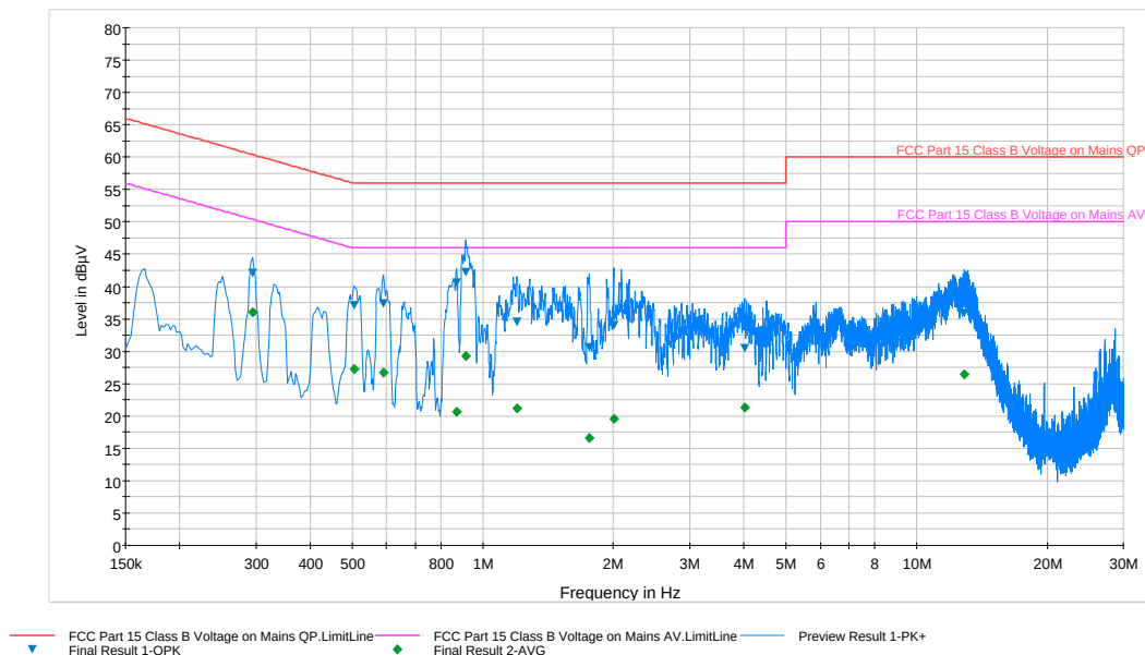
Plot 6-31. Line Conducted Plot with 802.11b (L1)
