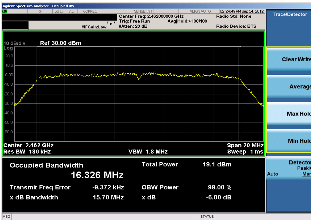
Plot 6-6. 6dB Bandwidth Plot (802.11g – Ch. 11)
