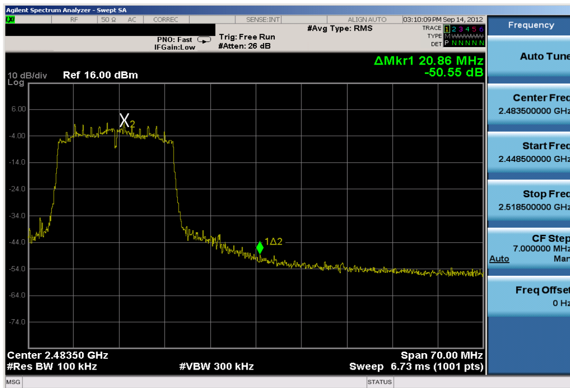
Plot 6-24. Band Edge Plot (802.11n – Ch. 11)
