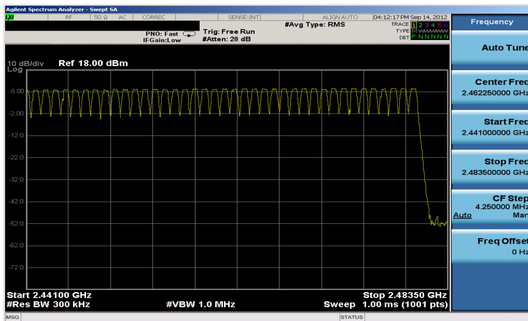
Plot 6-26. High End Spectrum Channel Hopping Plot (Bluetooth)
