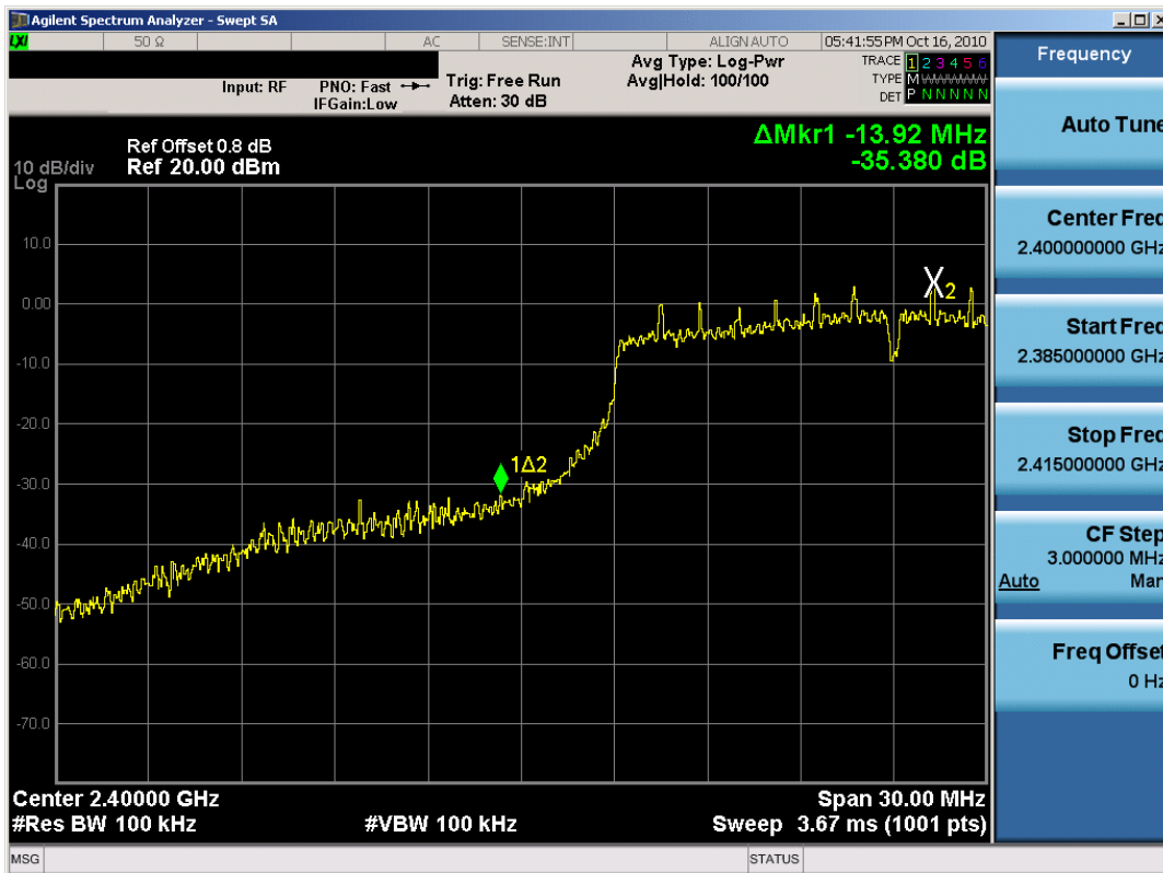
Plot 6-11. Band Edge Plot (802.11n – Ch. 1)
