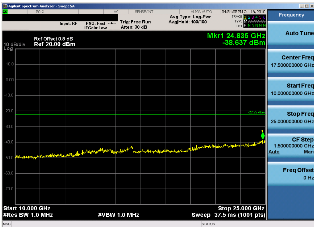
Plot 6-18. Conducted Spurious Plot (802.11b – Ch. 11)
