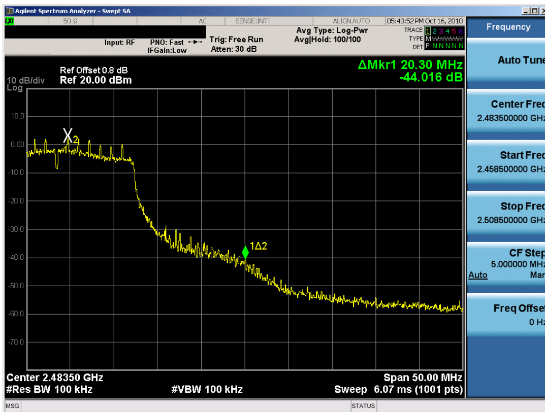
Plot 6-12. Band Edge Plot (802.11n – Ch. 11)
