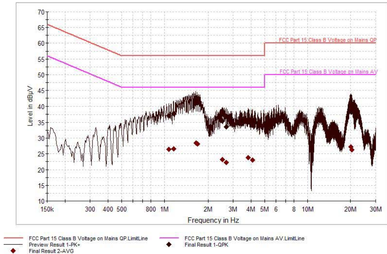
Plot 6-22. AC Line Conducted Plot with Bluetooth (Line 1)
