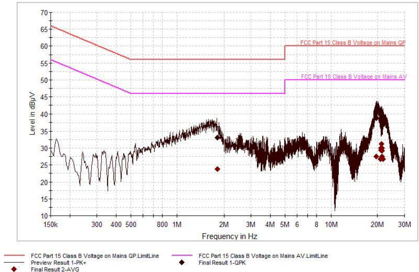
Plot 6-23. AC Line Conducted Plot with Bluetooth (Line 2(N))
