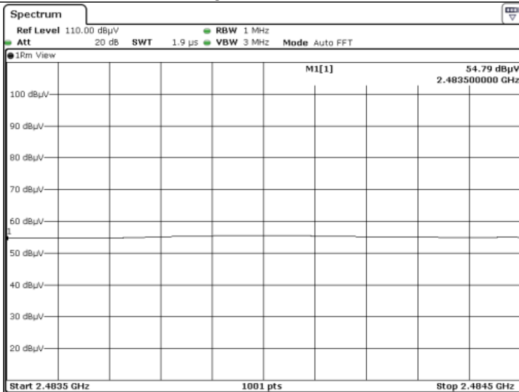
High Channel_Peak_V
