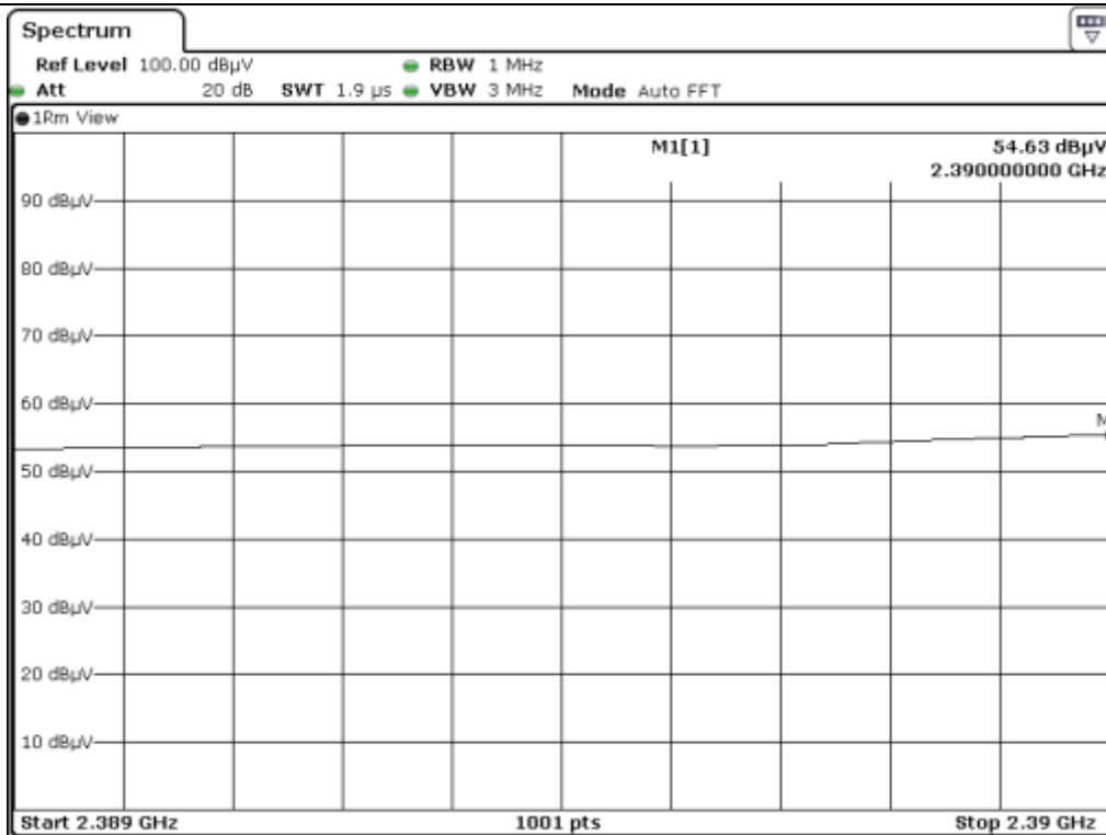
Low Channel_Peak_V
