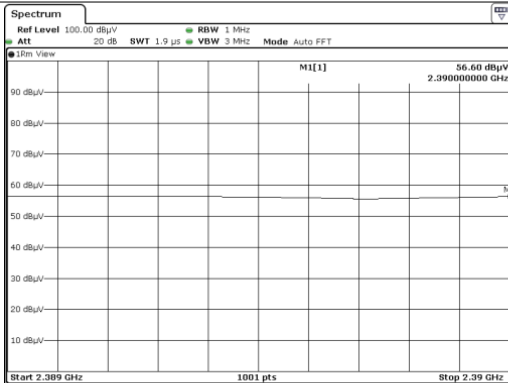
Low Channel_Peak_H
