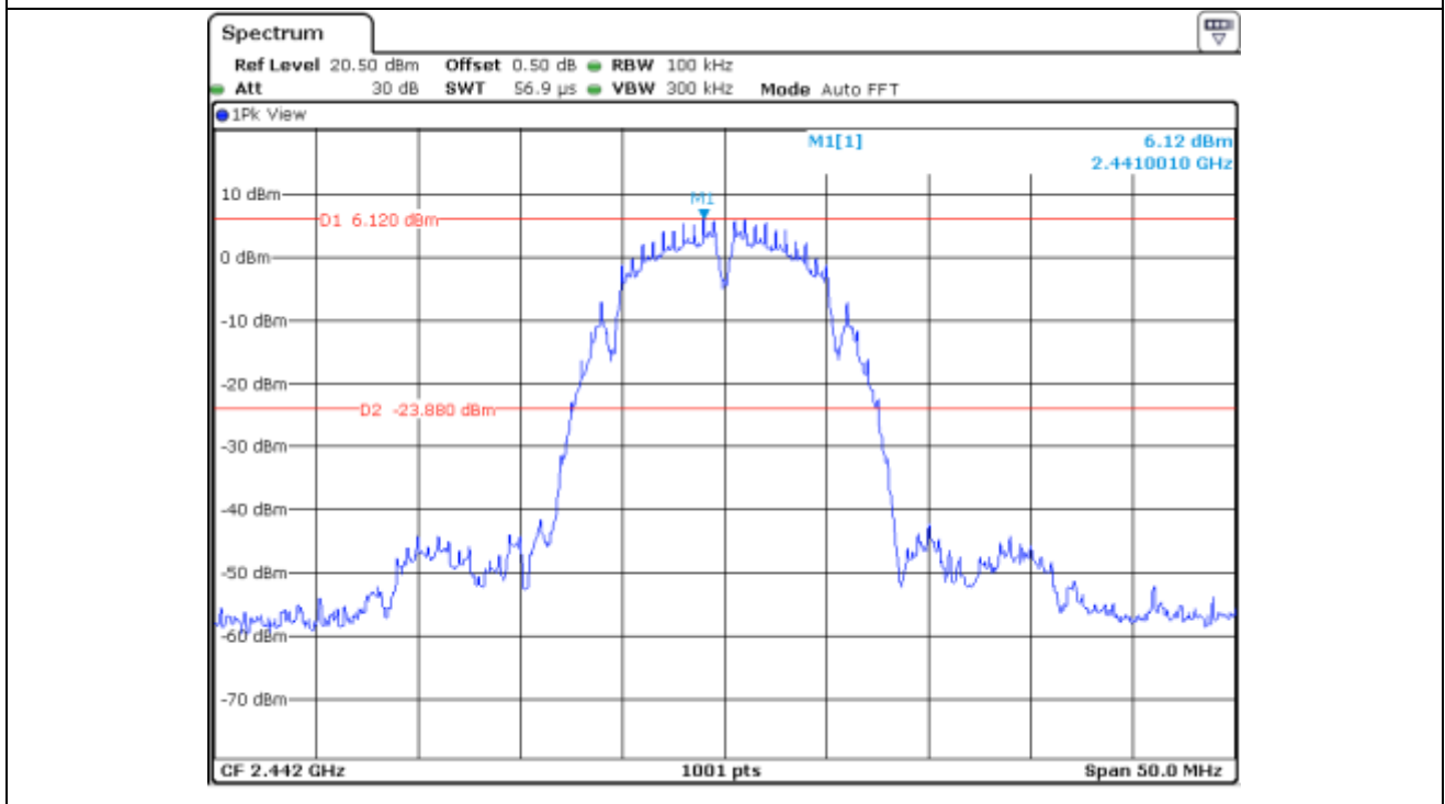
Middle Channel
