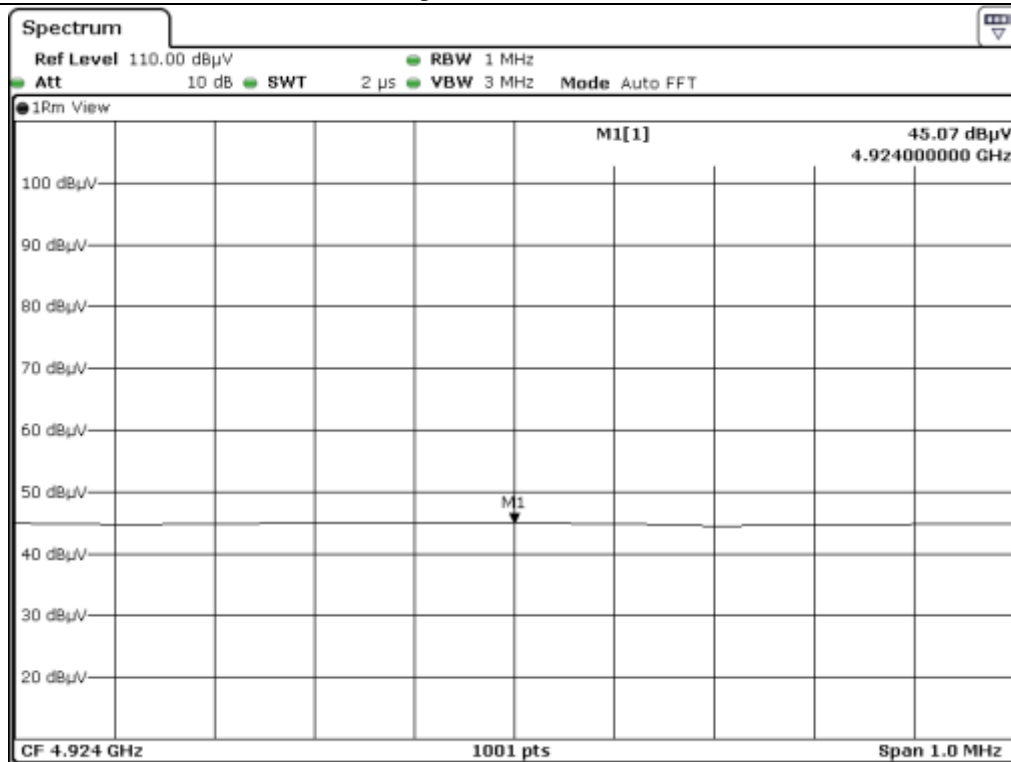
High Channel_Peak_V
