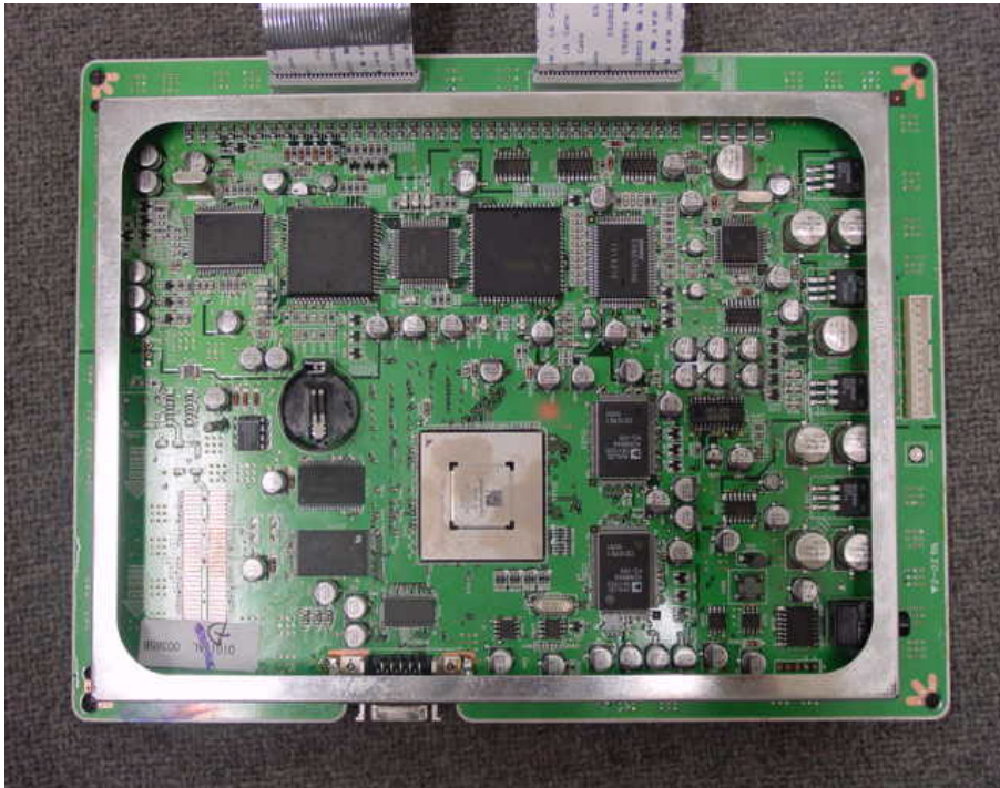
Rear view of Digital PCB
