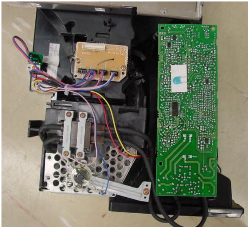
Rear view of Balast engine PCB
