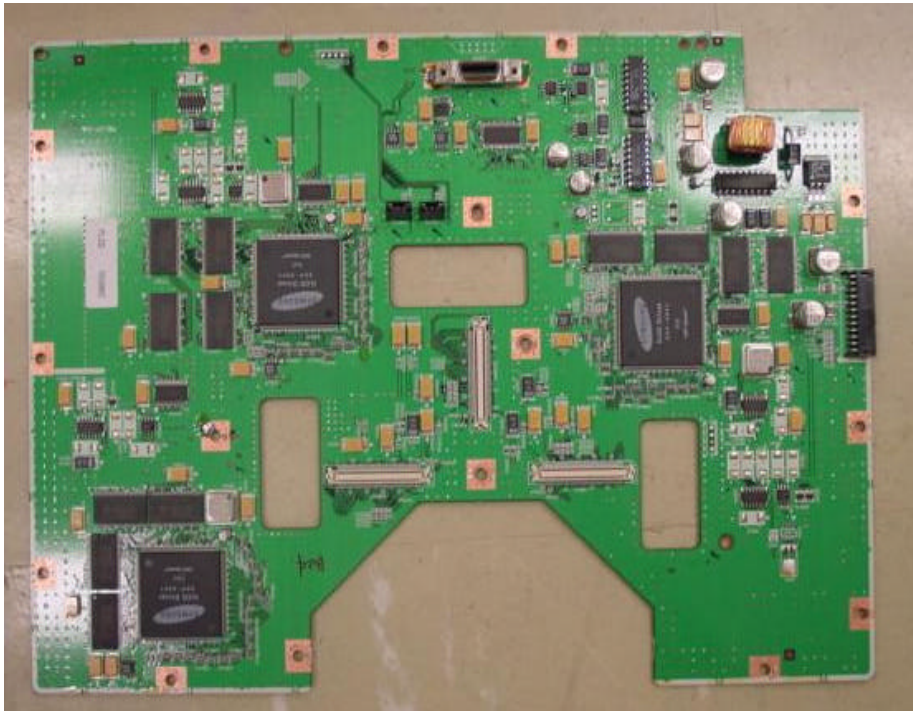
Front view of Drive PCB
