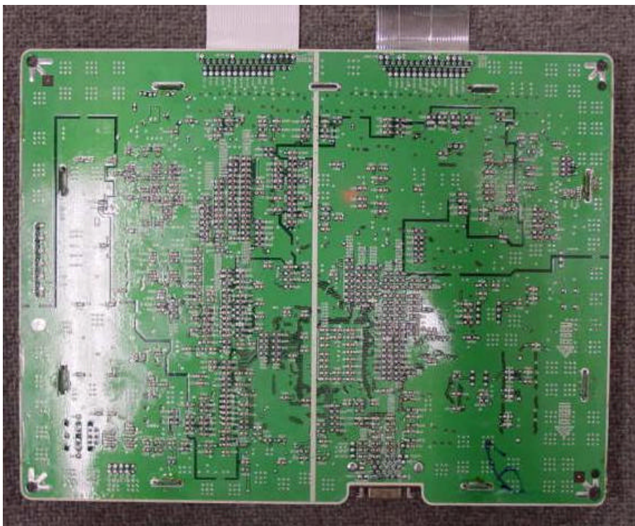
Rear view of Digital PCB
