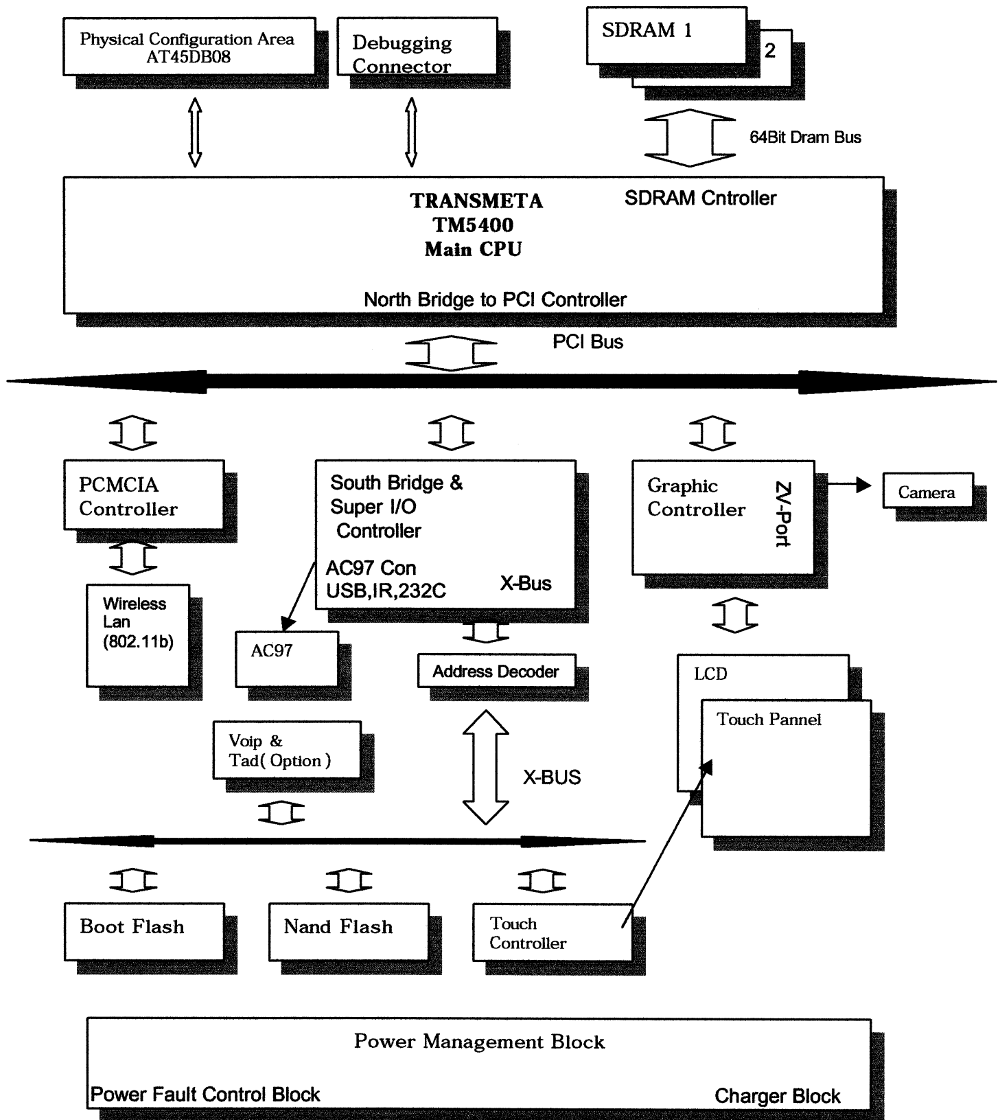
[ HomePad Block Diagram ]
