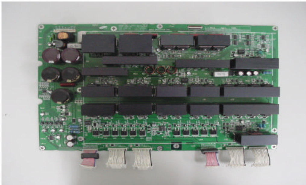
Y-DRIVER BOARD TOP VIEW
