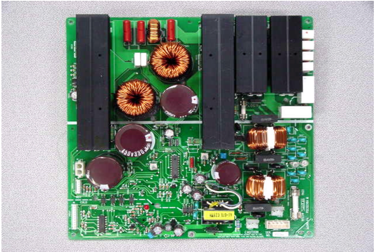
SMPS-1 board top view
