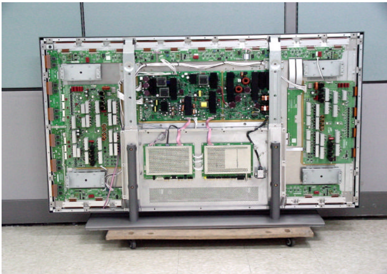
EUT Interior
