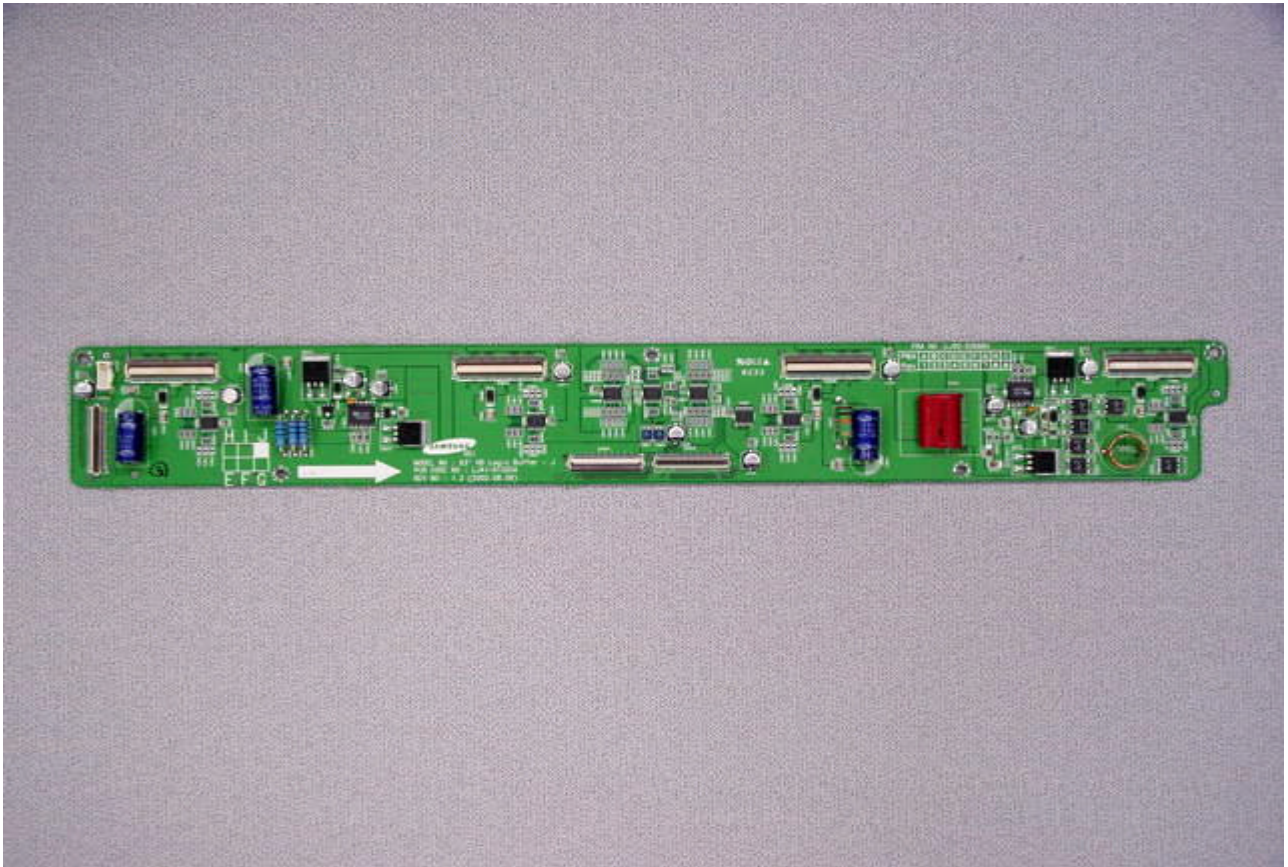
Logic buffer J board top view
