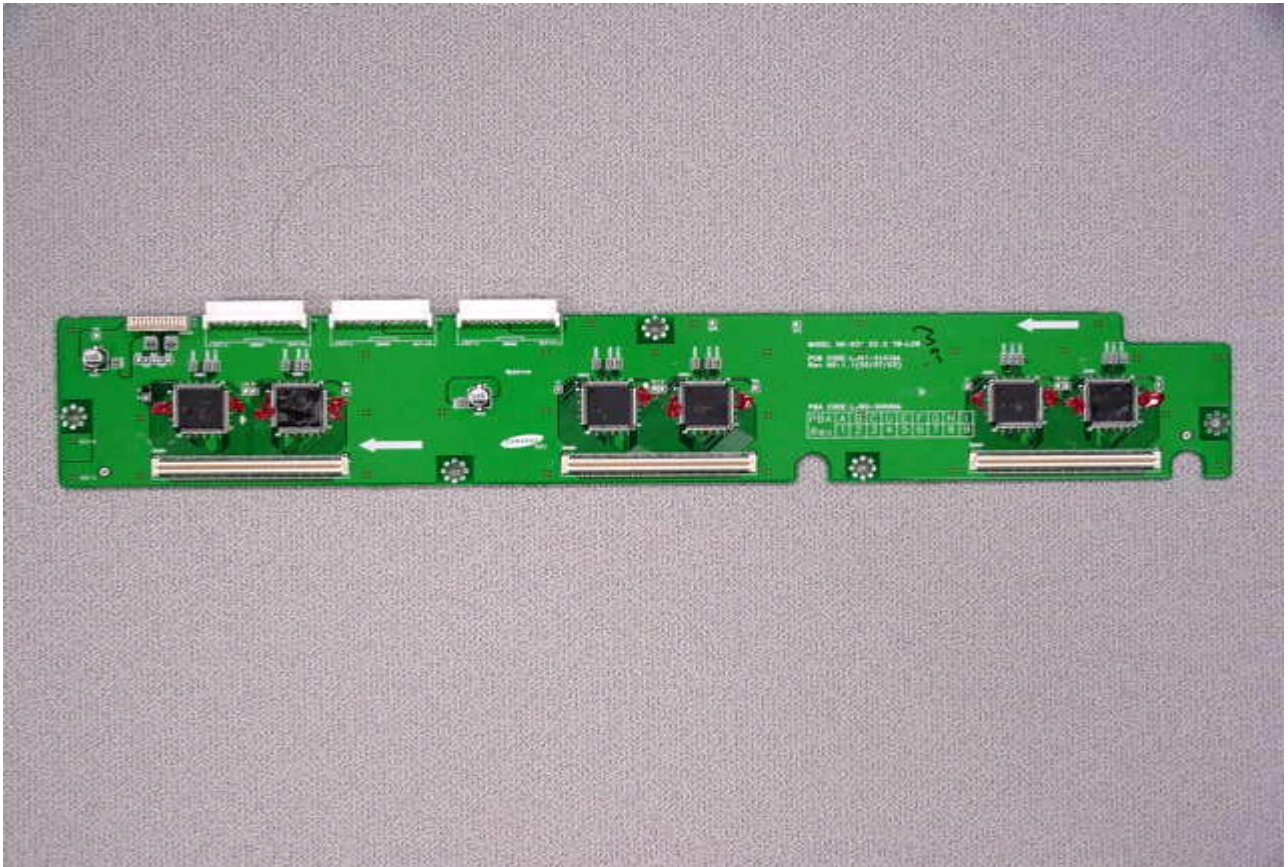
Address buffer board lower top view
