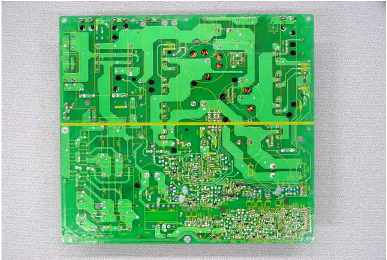
SMPS-2 board bottom view
