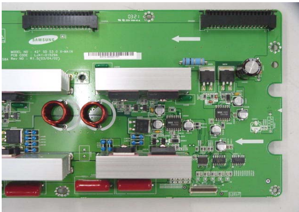
X driver board-1 top view
