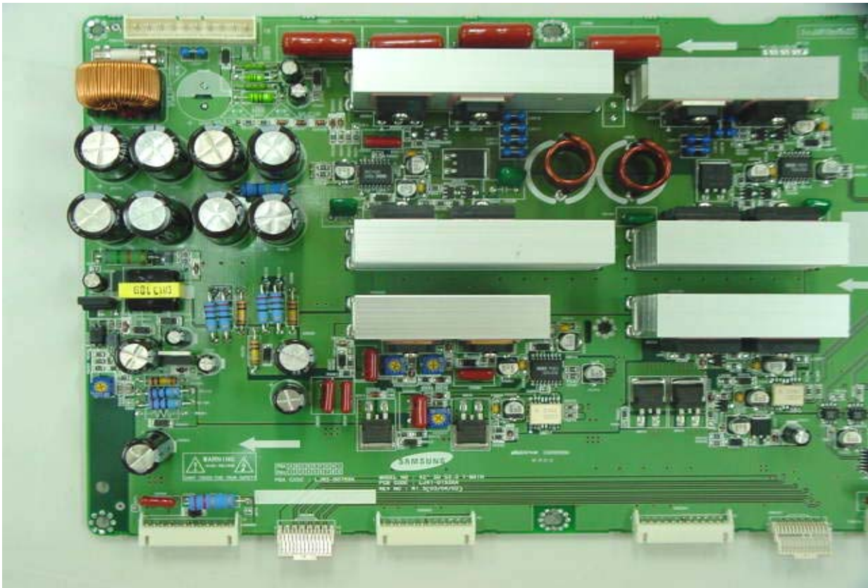
Y driver board top view
