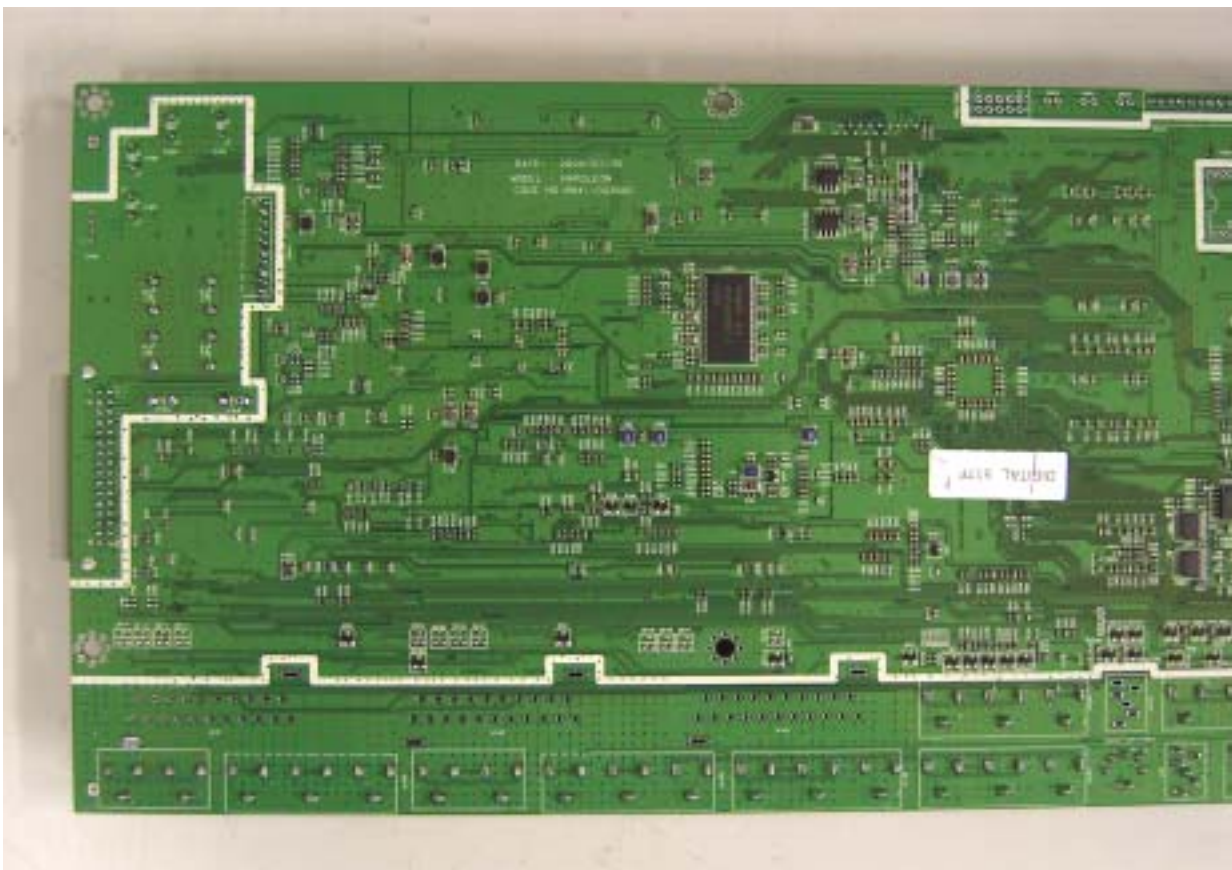
Digital board-1 bottom view
