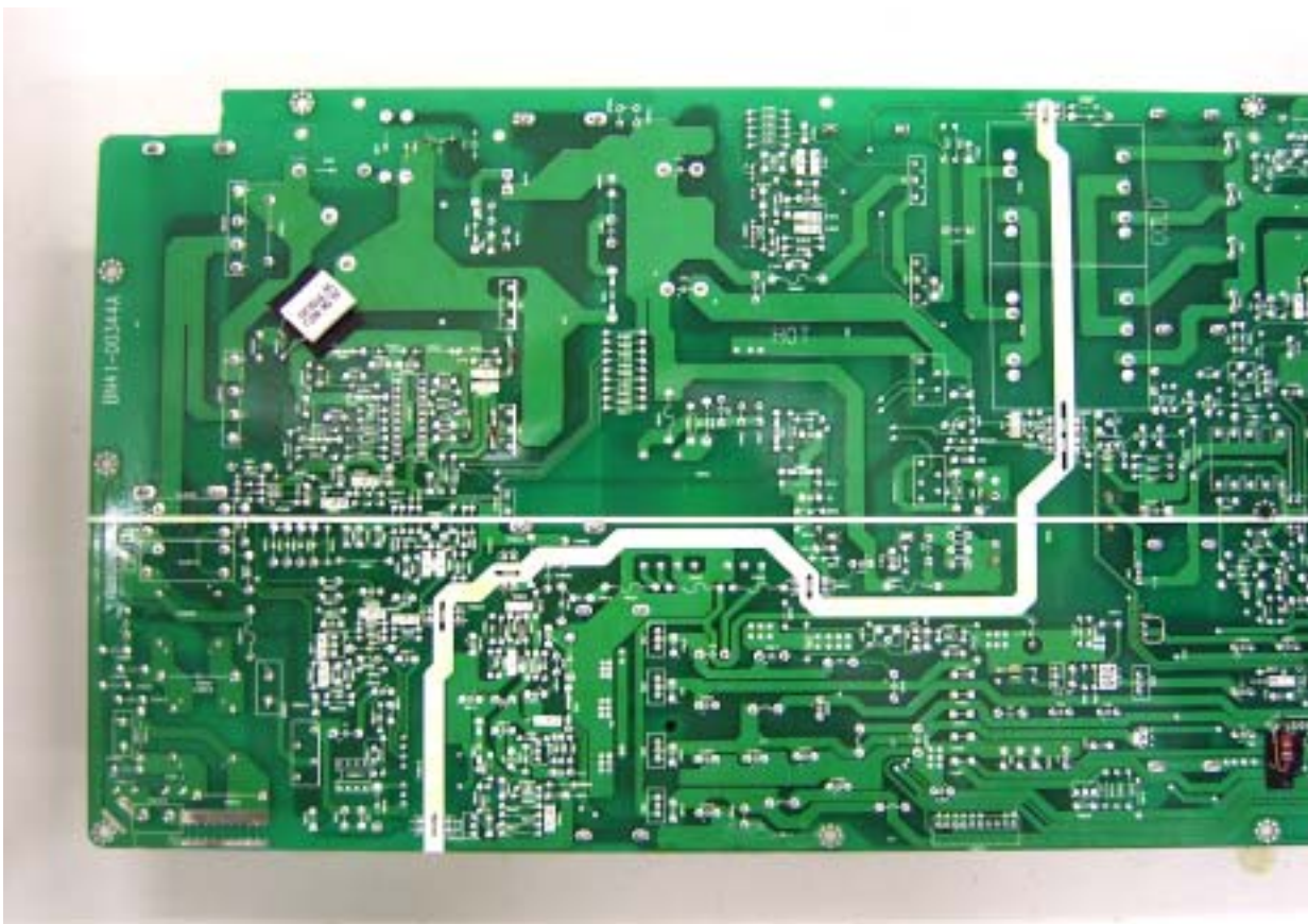
SMPS board bottom view-2
