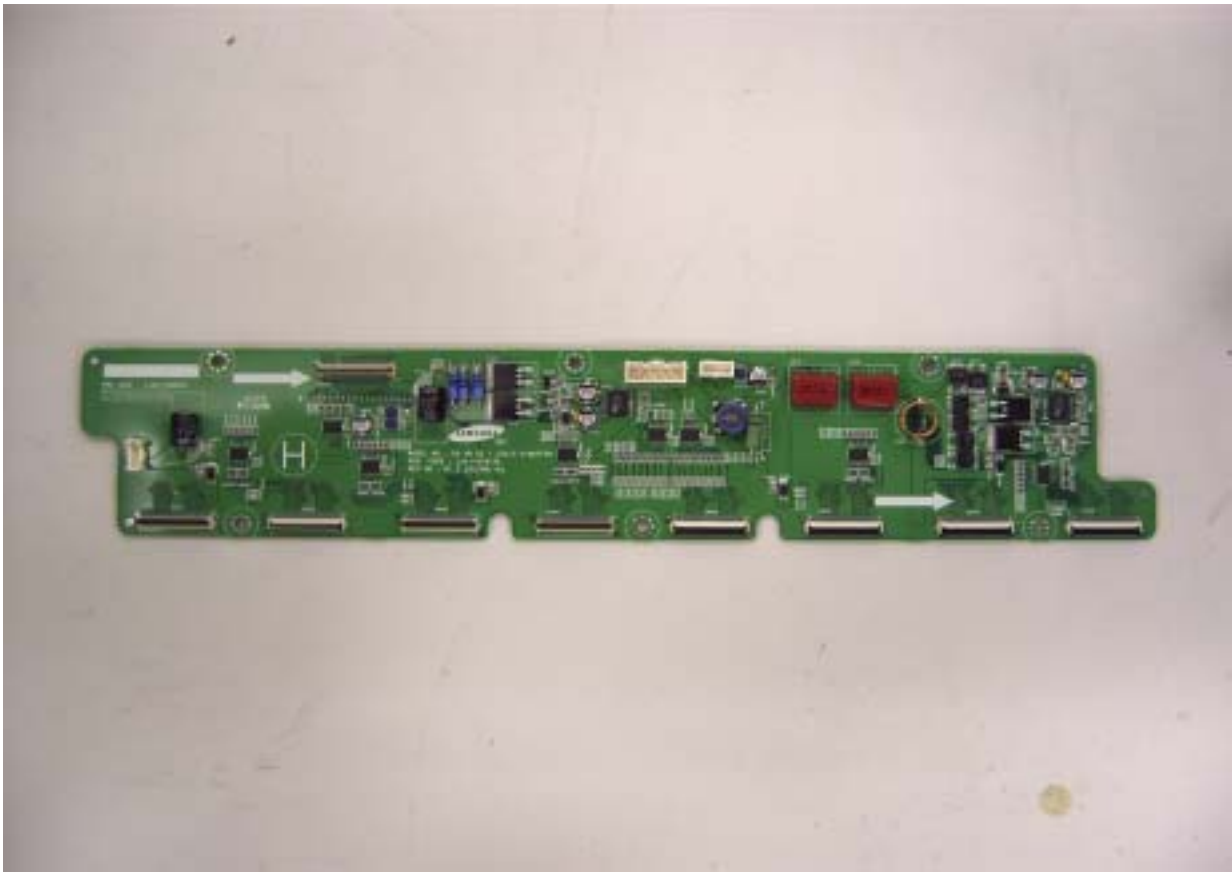
H buffer board top view
