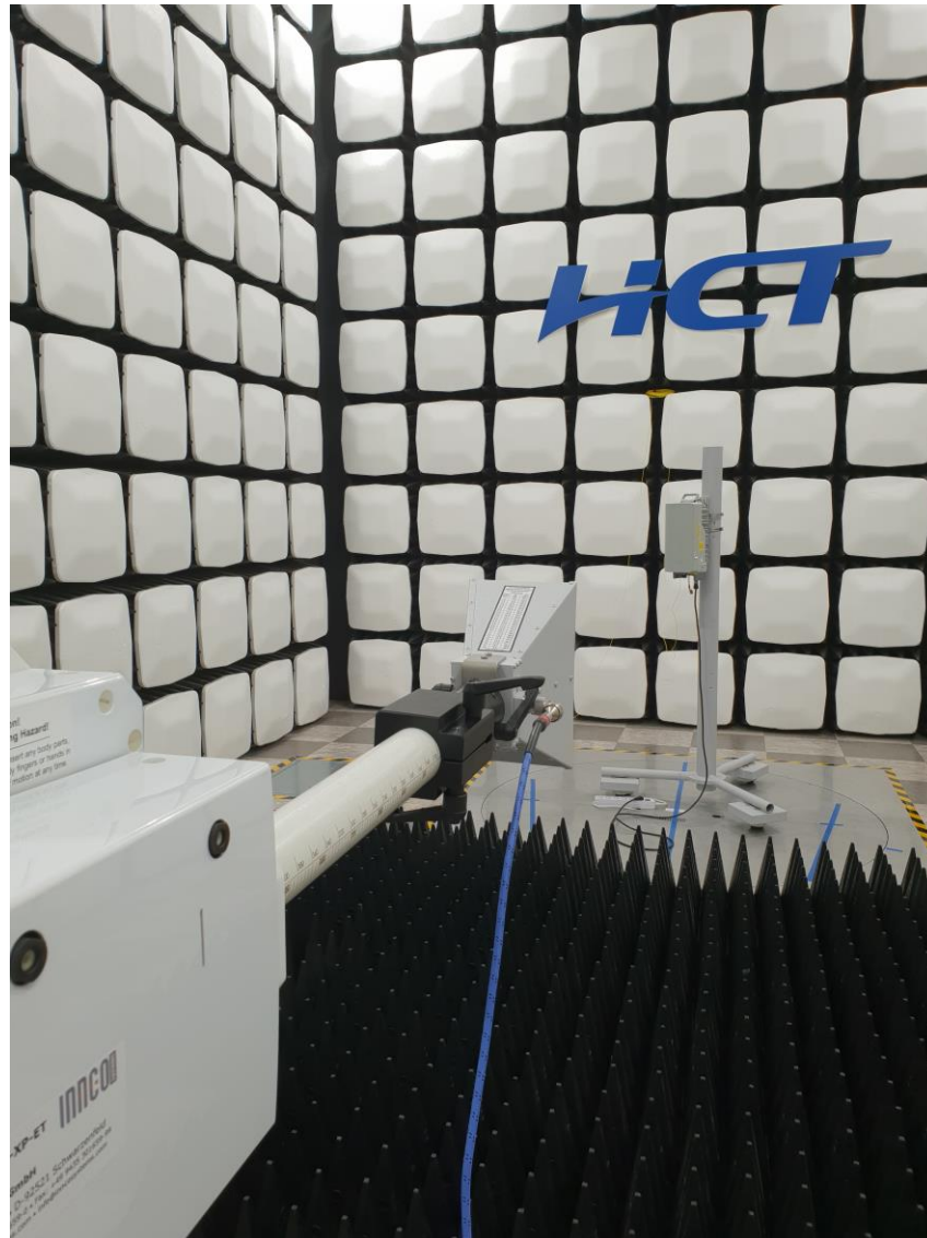
Radiated Test Setup Photo – Spurious (Horn Antenna 1 GHz ~ 18 GHz, Horizontal)
