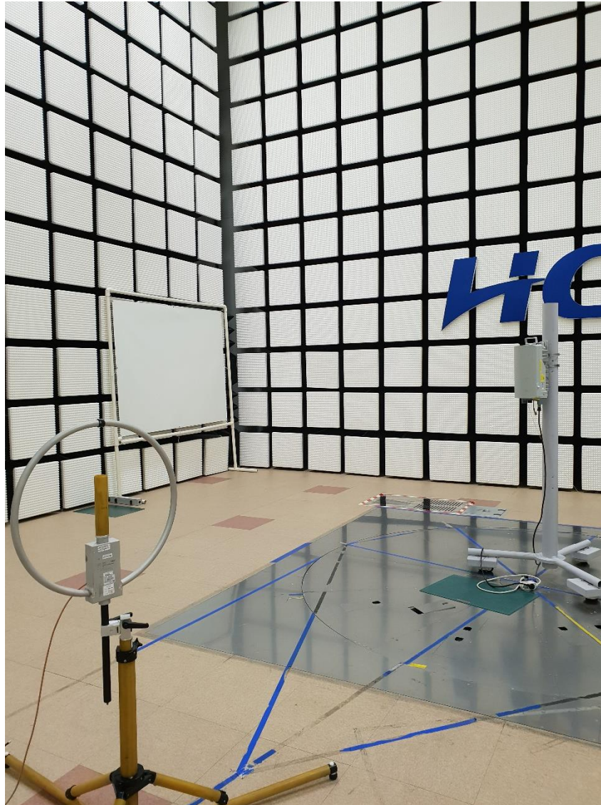
Radiated Test Setup Photo –Spurious (Loop Antenna, Vertical)
