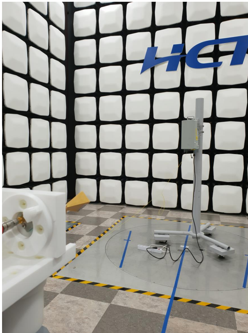
Radiated Test Setup Photo – Spurious (WR-12 Horn Antenna, Upper)
