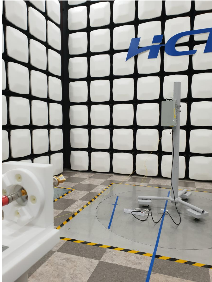
Radiated Test Setup Photo – Spurious (WR-05 Horn Antenna, Lower)
