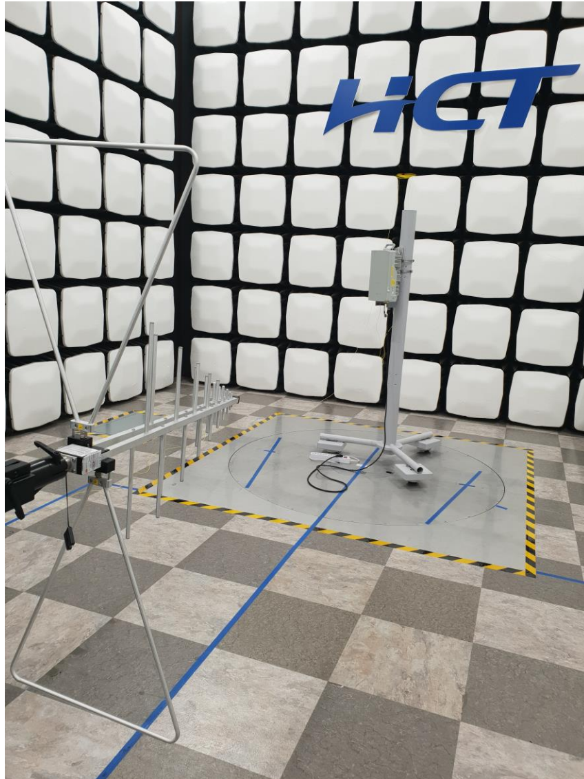
Radiated Test Setup Photo – Spurious (Bi-log Antenna, Vertical)
