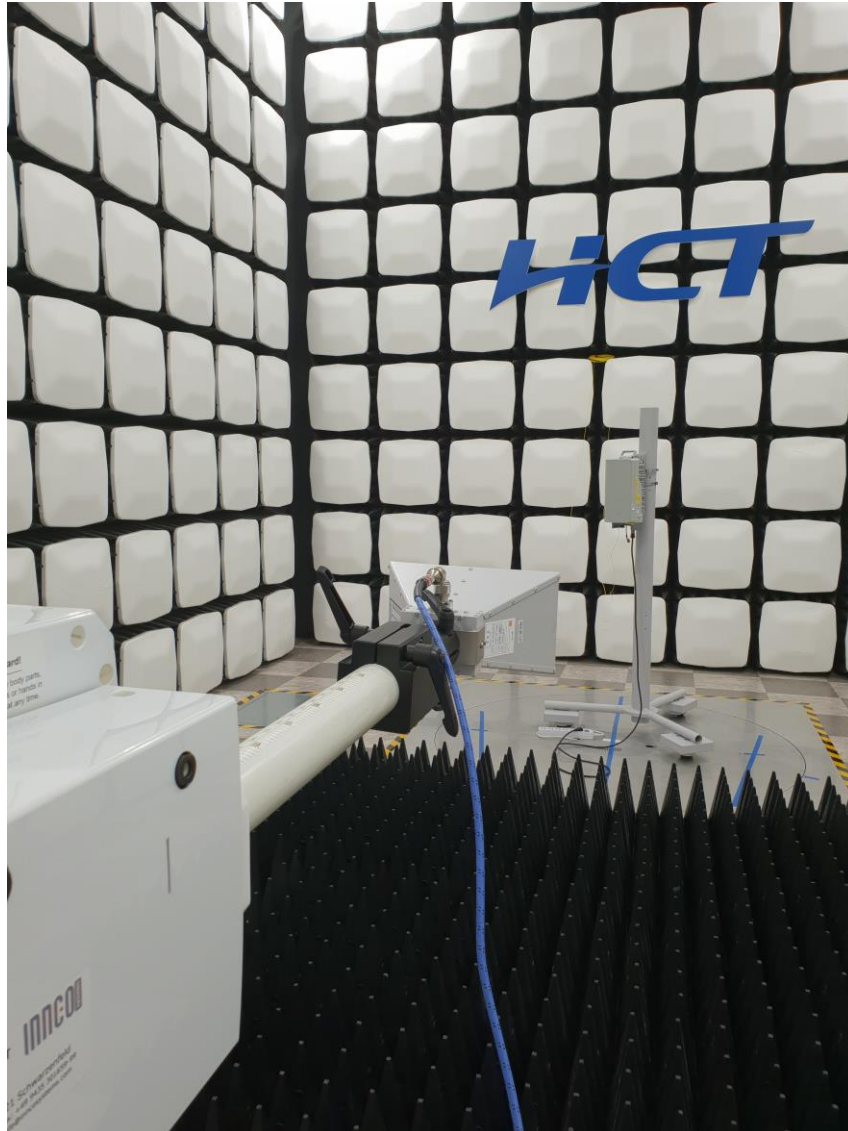
Radiated Test Setup Photo – Spurious (Horn Antenna 1 GHz ~ 18 GHz, Vertical)
