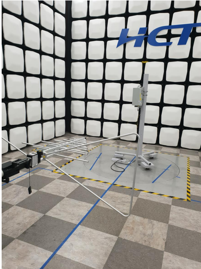
Radiated Test Setup Photo – Spurious (Bi-log Antenna, Horizontal)
