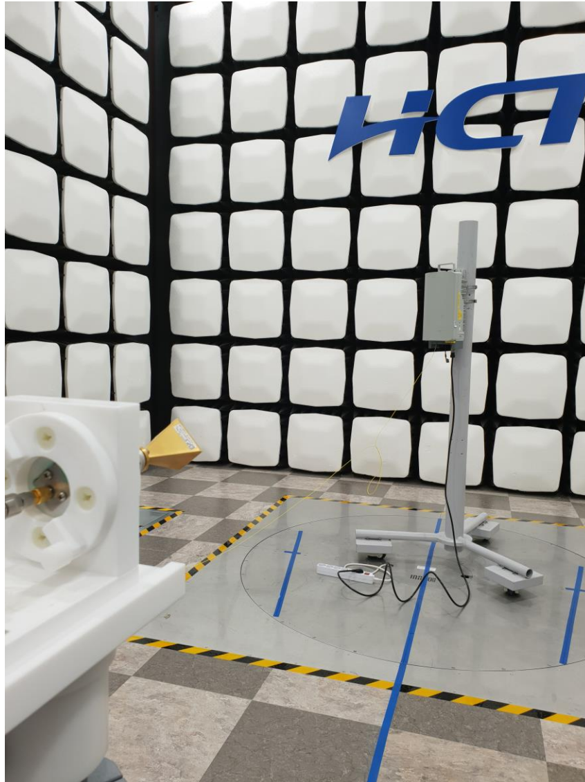
Radiated Test Setup Photo – Spurious (WR-12 Horn Antenna, Lower)
