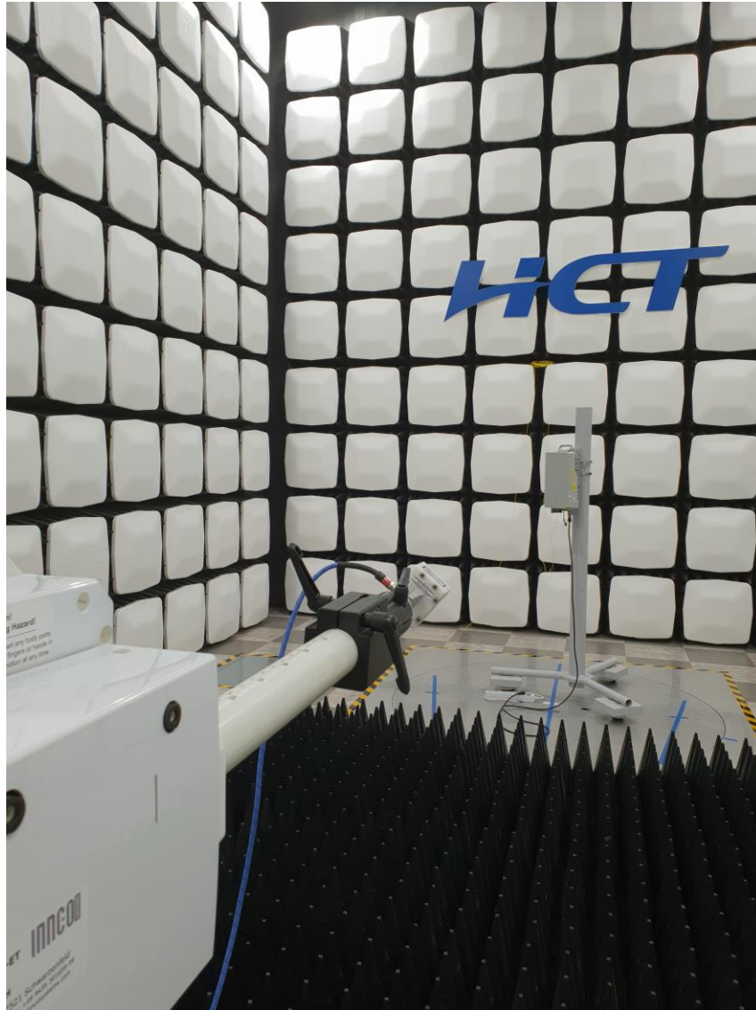
Radiated Test Setup Photo –Spurious (Horn Antenna 18 GHz ~ 40 GHz, Upper)
