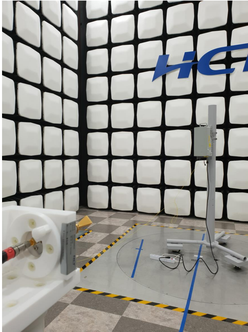
Radiated Test Setup Photo – Spurious (WR-08 Horn Antenna, Upper)
