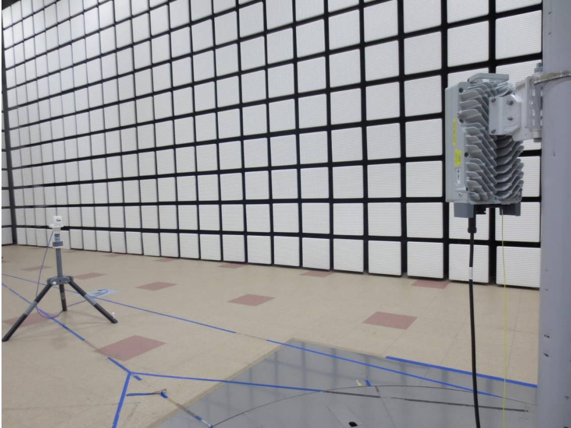
Radiated Test Setup Photo – Spurious (140 GHz ~ 200 GHz, (135°))
