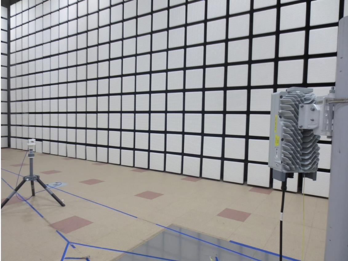
Radiated Test Setup Photo – Spurious (90 GHz ~ 140 GHz, (45°))
