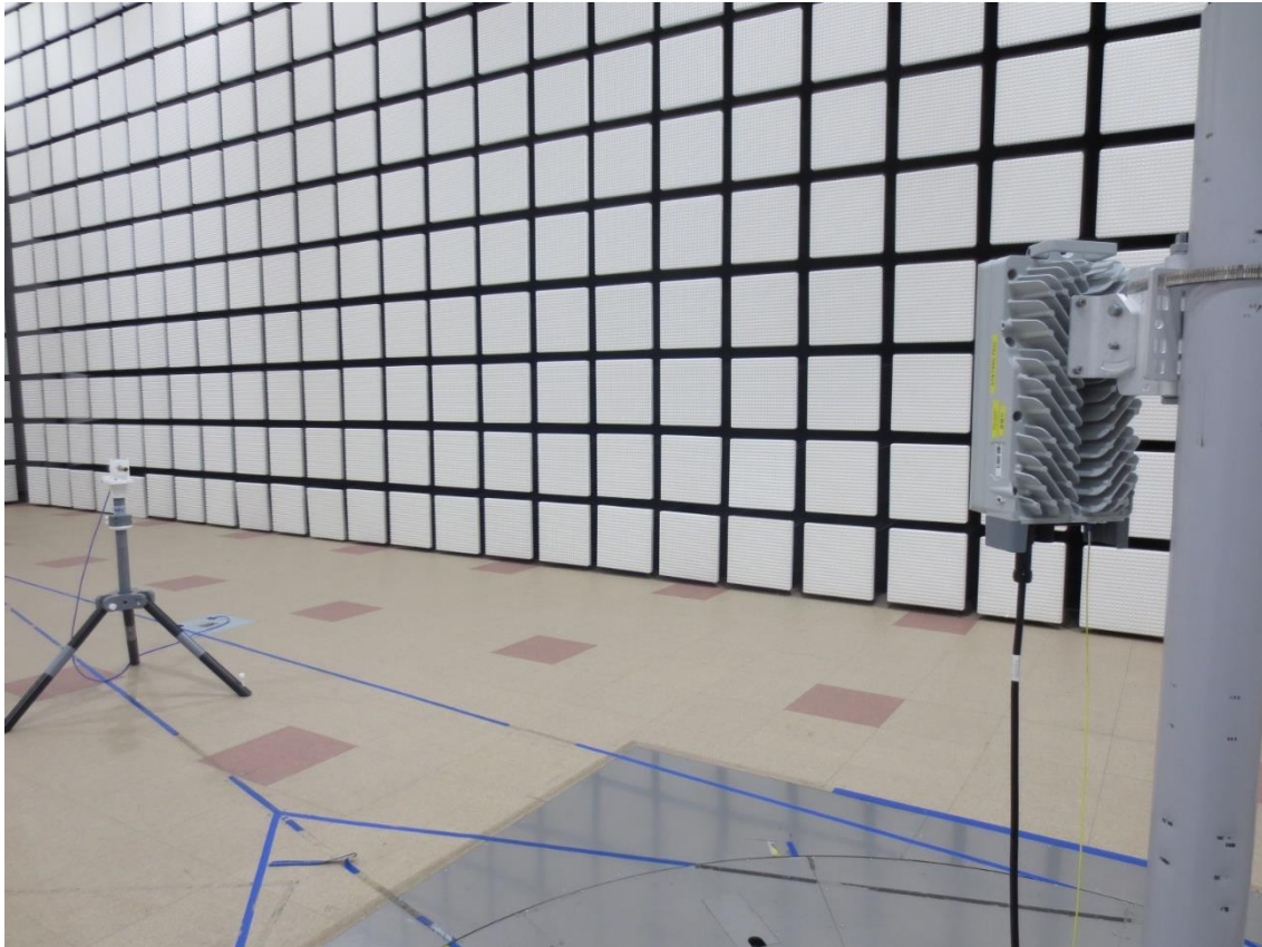
Radiated Test Setup Photo – Spurious (90 GHz ~ 140 GHz, (135°))
