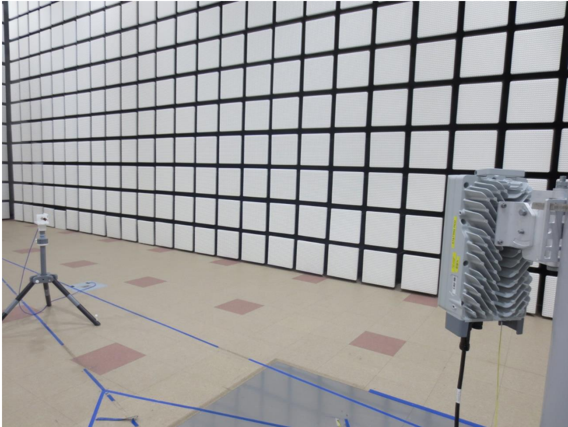
Radiated Test Setup Photo – Spurious (60 GHz ~ 90 GHz, (45°))
