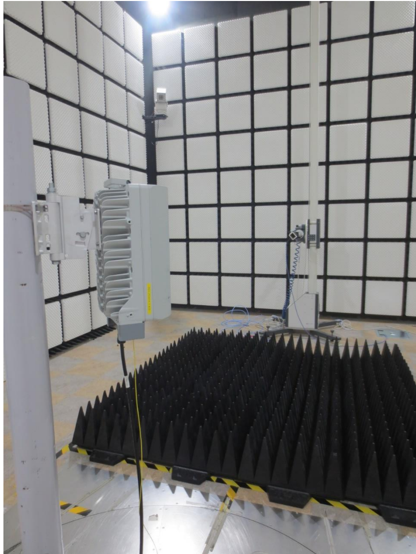
Radiated Test Setup Photo –Spurious (18 GHz ~ 40 GHz band (45°))
