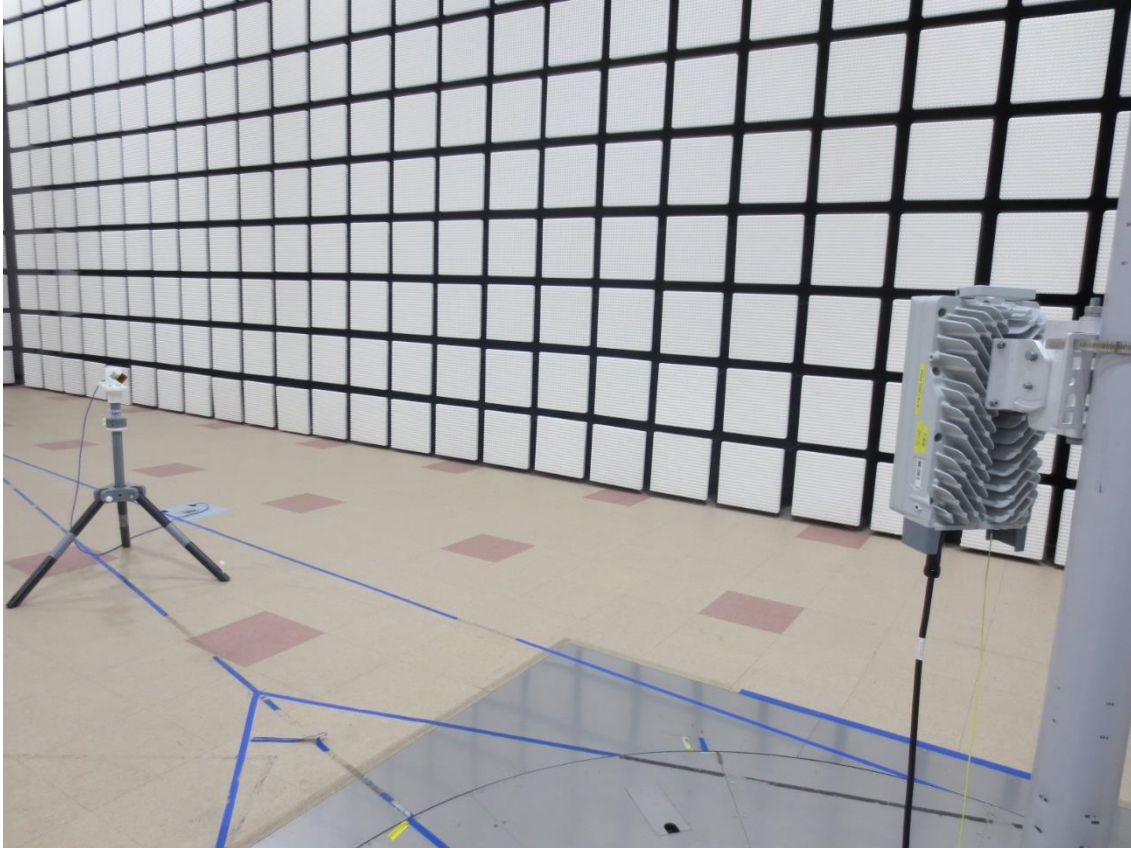
Radiated Test Setup Photo – Spurious (40 GHz ~ 60 GHz, (135°))
