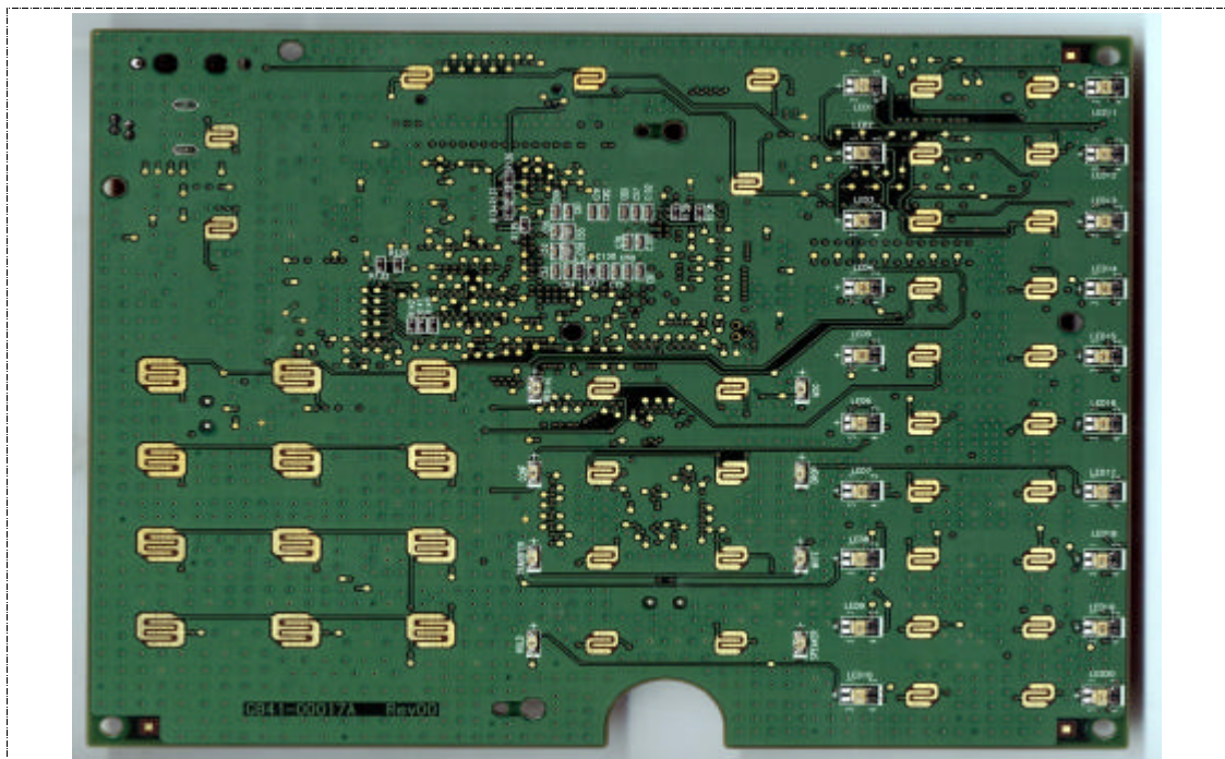
Solder view of main b'd
