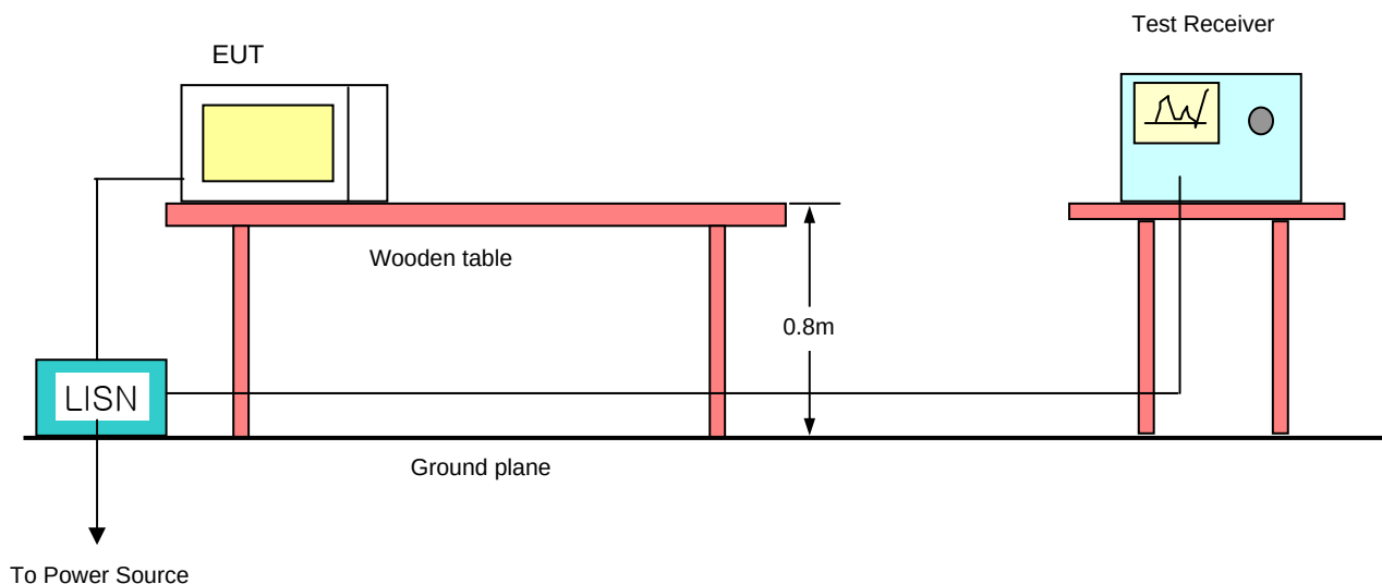
Fig. 5 Conducted Emission Configuration(0.15 - 30MHz)
