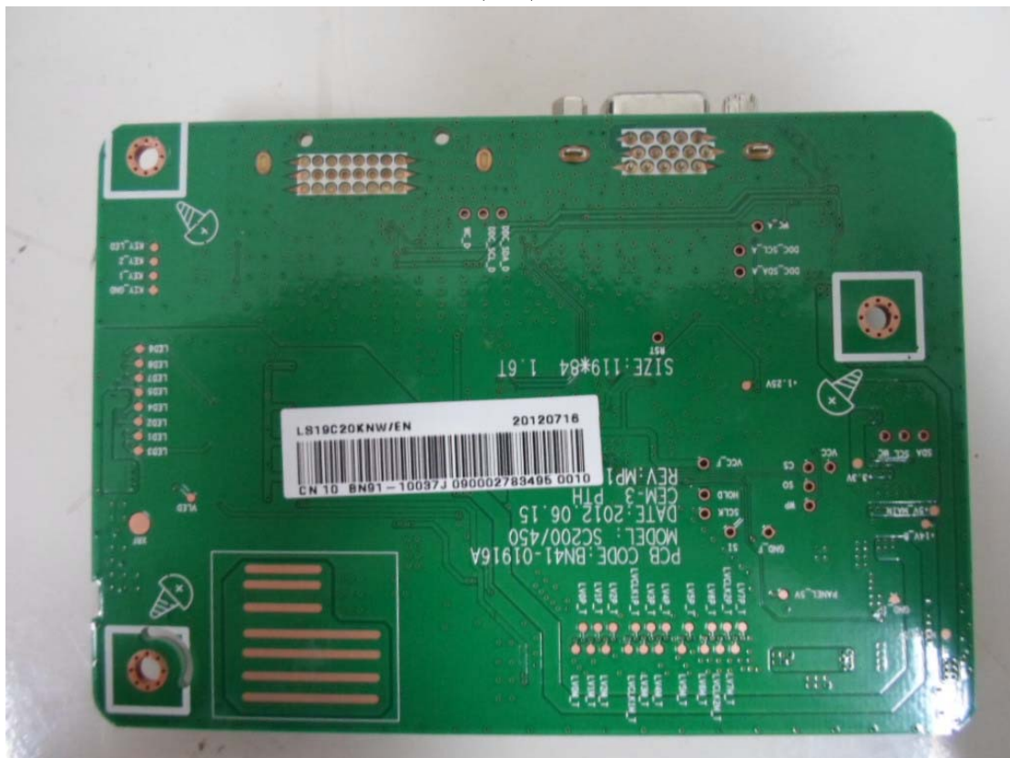
back change BN41-01916A(new) internal rear view
