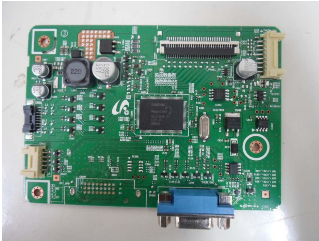
back change BN41-01916A(new) internal front view
