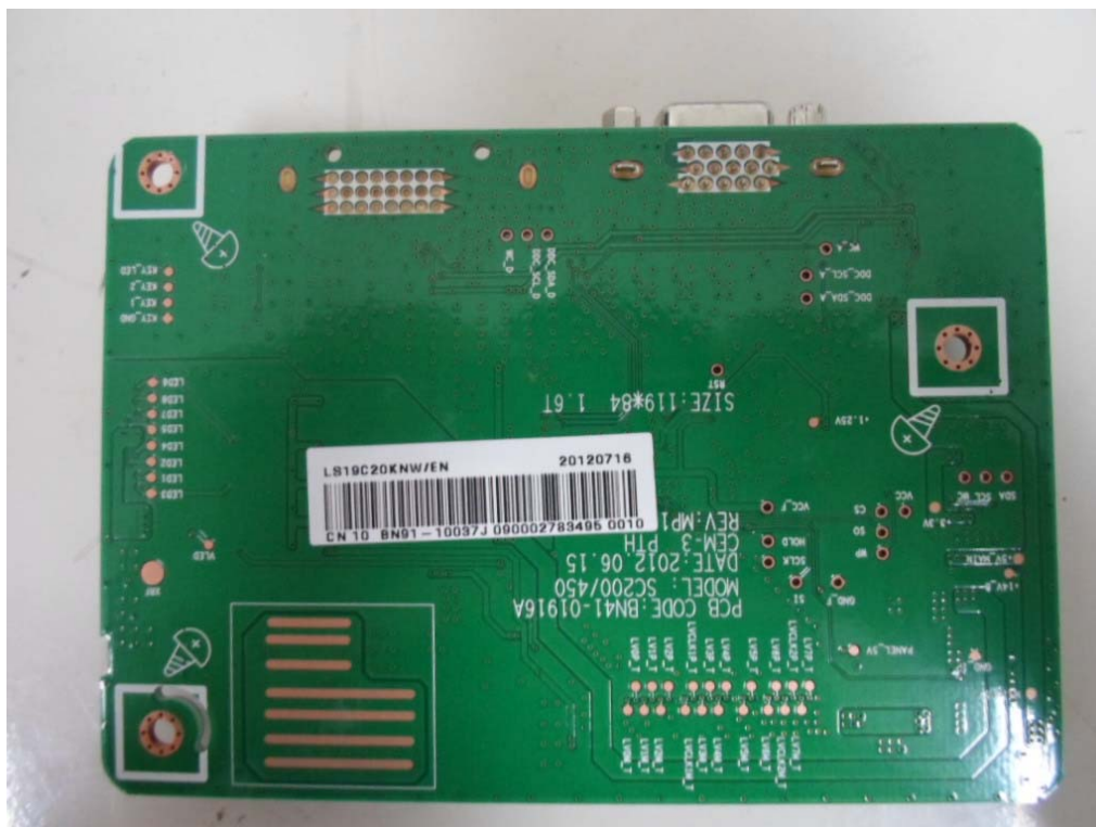
before change BN41-01916A (old) rear view
