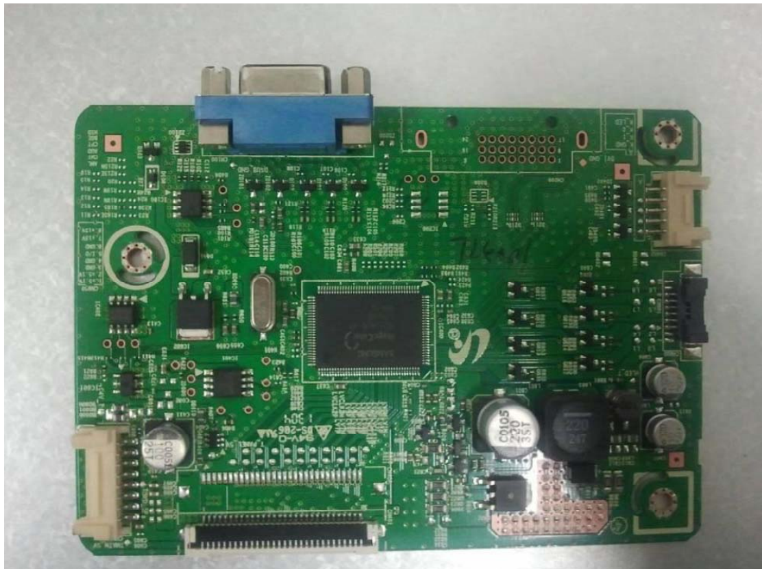
back change BN41-01916A (new) front view
