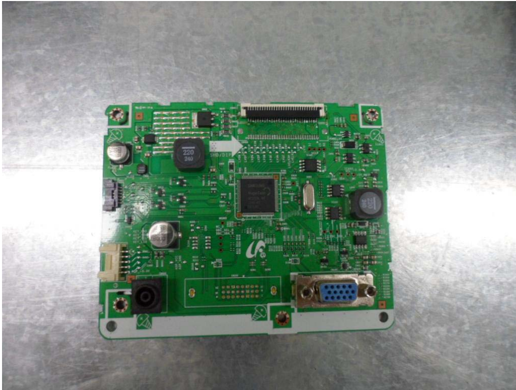
after change BN41-01967A(VGA) Internal front view
