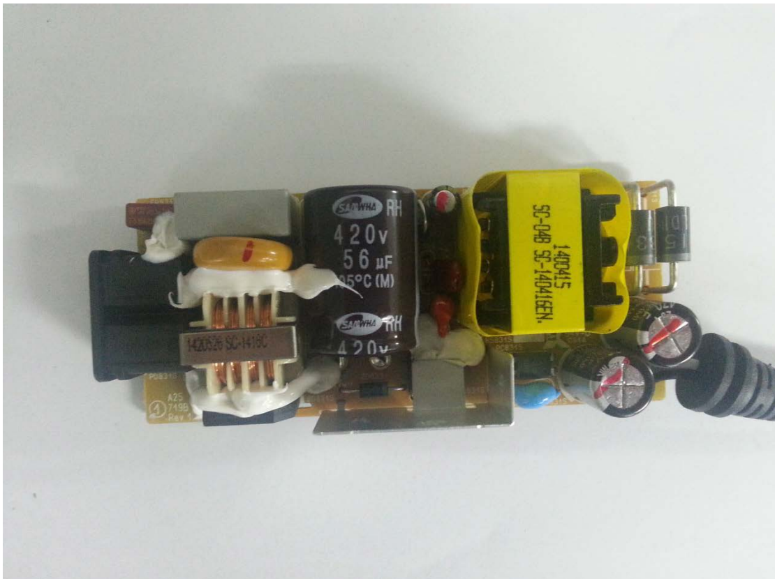
Before change A2514_DPN internal rear view
