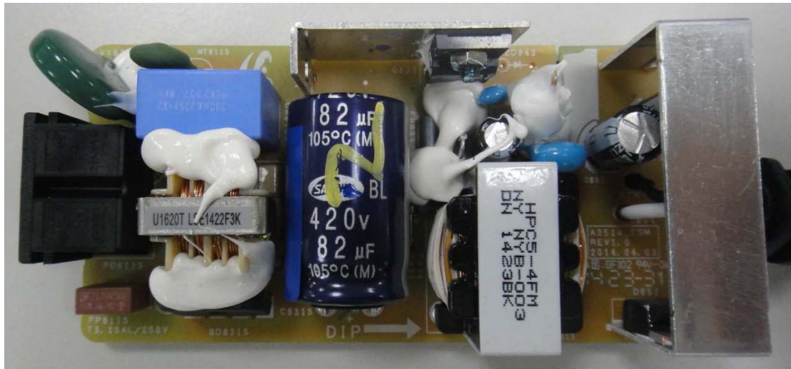
Back change A3514_ESM internal front view
