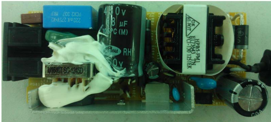
Before change A2514_DSM internal rear view
