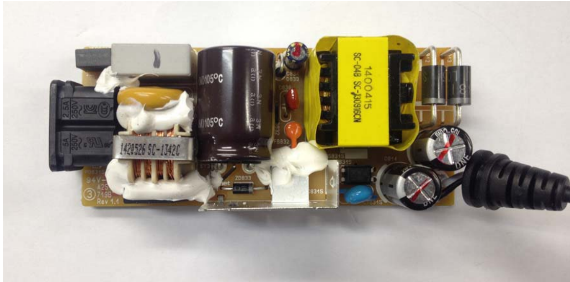
Before change A2514_DPN internal front view
